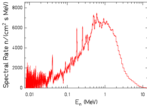
FIG. 2. Neutron spectral rate measured with the H19 fission chamber from PTB at a flight path length of 618 cm. The electron beam energy and current were 31 MeV and 15 \mu A, respectively.
