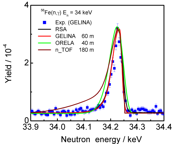
FIG. 4. The experimental yield in the region of the 34 keV resonance of ^{56}\text{Fe} obtained at a 60 m station of GELINA. The yield is compared with the result of a RSA. The response functions of GELINA, n_TOF and ORELA are also given.
