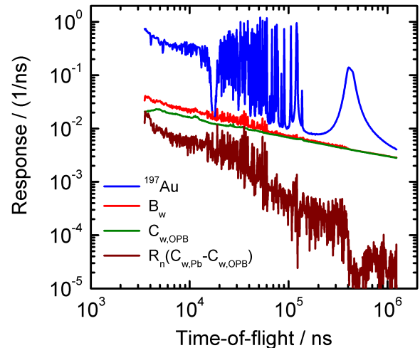
FIG. 22. The response of a C_6D_6 detector system as a function of TOF for a 1.0 mm ^{197}\text{Au} sample [198] obtained at GELINA is compared with the contribution of the different background components.
