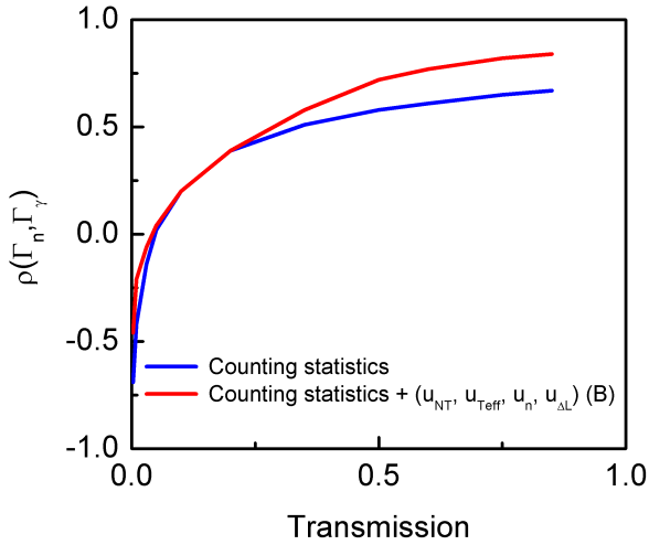
FIG. 29. The correlation coefficient \rho(\Gamma_n, \Gamma_\gamma) as a function of transmission. The coefficient is given for an analysis accounting only for counting statistics and for additional uncertainties due to normalization N_T , temperature T_{eff} , resolution broadening \Delta L and area density n , obtained by CUP.
