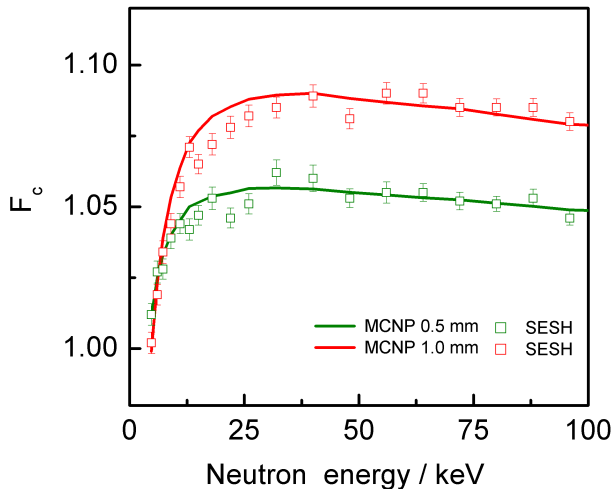
FIG. 10. Factors F_c , to correct for self-shielding and multiple interaction events, for a 0.5 mm and 1.0 mm thick ^{197}\text{Au} sample obtained with SESH are compared with those from MCNP/NJOY.
