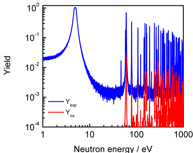
FIG. 21. The experimental yield as a function of neutron energy for a 0.122 mm thick Au sample is compared with the background contribution due to the neutron sensitivity of the detector ( Y_{ns} ). The data result from measurements with the BaF 2 detector at n_TOF [99].
