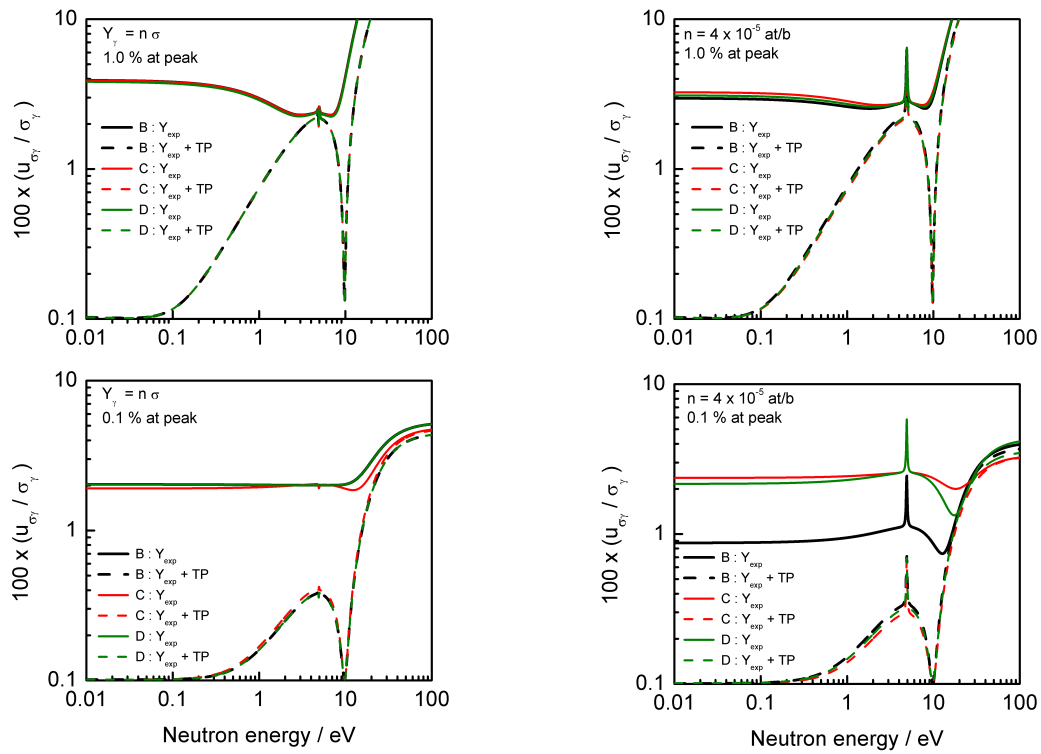
FIG. 27. The relative uncertainty of the capture cross section obtained from parameters which were derived from different experimental data sets. The data base consisted of experimental yields and an accurate capture cross section at 0.0253 eV (TP). The cross section was supposed to be the sum of a contribution of a s-wave resonance at 4.9 eV and a 1/v -contribution.
