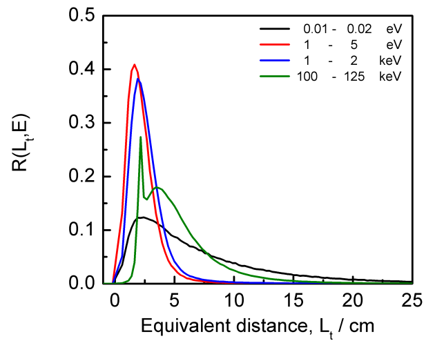
FIG. 2. The probability distribution of the equivalent distance L_t that a neutron travels in the target-moderator assembly of GELINA.
