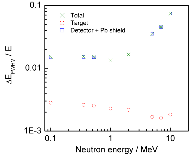
FIG. 5. The total energy resolution (at FWHM) ( \times ) for transmission measurements at nELBE together with the contribution due to the neutron target ( \circ ) and the one from a 1.1 cm thick plastic scintillator [58] including a 1 cm Pb shield ( \square ).
