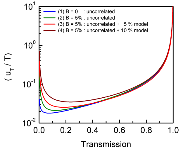
FIG. 15. The calculated relative uncertainty as a function of transmission for different background conditions and contributing uncertainty components (see text).
