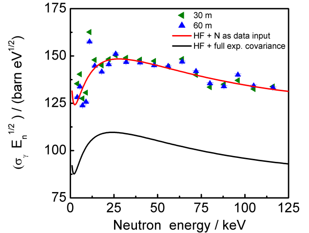
FIG. 26. The average capture cross section (multiplied by E_n^{1/2} ) for ^{103}\text{Rh} as a function of neutron energy derived from measurements at GELINA [209]. The results of a least squares adjustment are also given (see text).
