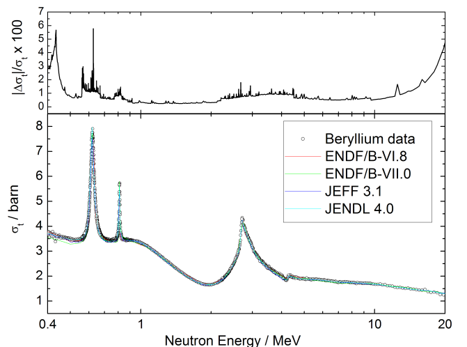
FIG. 13. Results of transmission measurements on Be performed at RPI are compared with the data in the evaluated data files.
