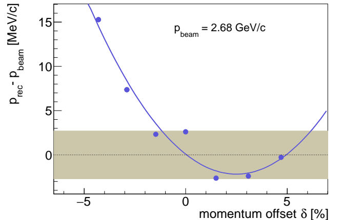
Fig. 16. (Color online) Absolute error on proton momenta ( p_{rec} - p_{beam} ) for seven different spectrometer beam line settings. Statistical errors are negligible. The error band represents the magnitude of systematic errors due to uncontrolled primary beam positions on the production target. The curve is the result of a parabolic fit.
