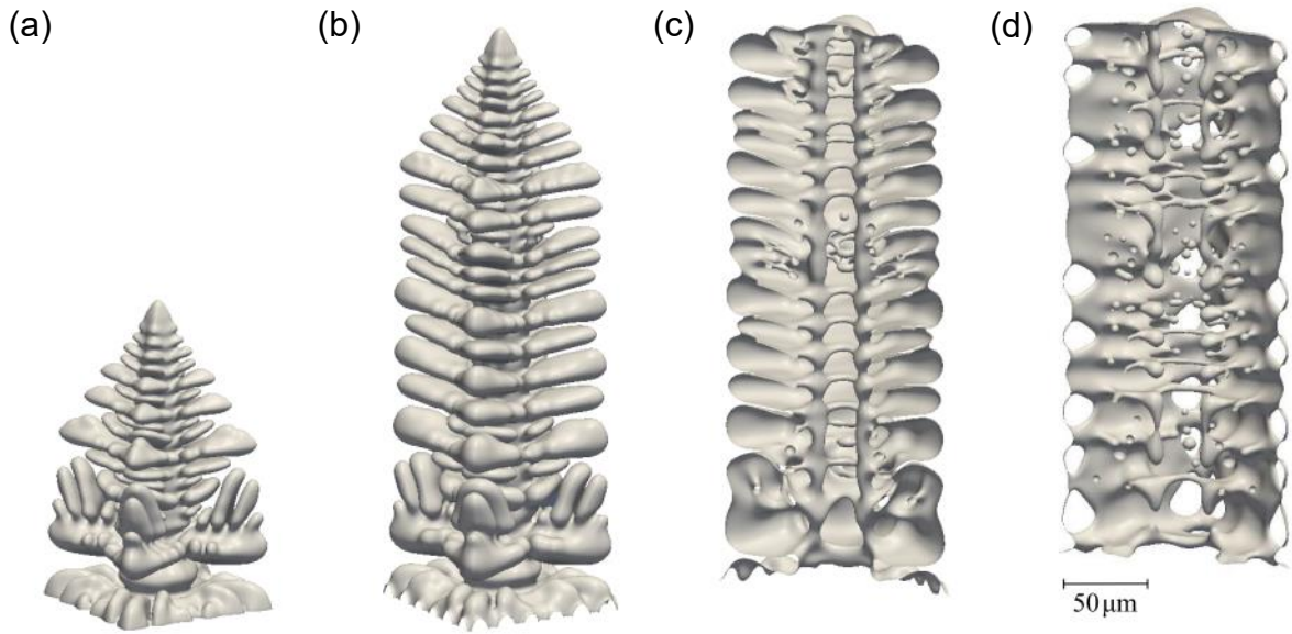
Fig. 2. Evolution of the dendrite geometry for the base case simulation: full view of the growing dendrite at t = 0.5 s (a) and 1 s (b); cutaway view of half of the dendrite at t = 2.5 s (c) and 7 s (d) [2].
