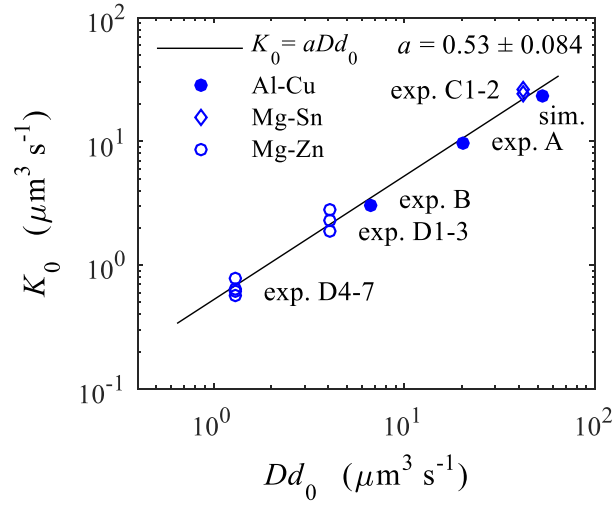
Fig. 8. Variation of the rate constant K_0 with alloy properties D_d d_0 , using r = 0.4 for the simulations and r = 0.25 for the experiments.
