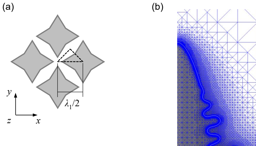
Fig. 1. Computational model: (a) assumed arrangement of the dendrites normal to the temperature gradient and triangular cross section of the calculation domain; (b) example of the adaptive mesh refinement used near the solid-liquid interface.
