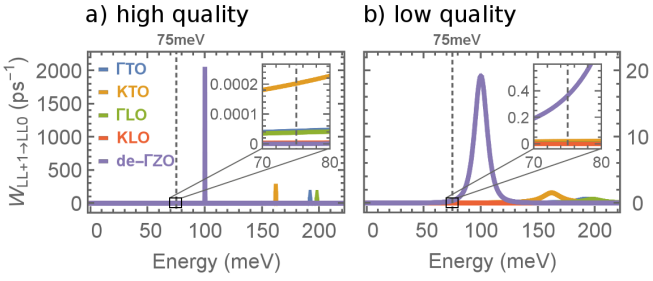
Figure 3. Scattering rates induced by different phonon modes in dependence of the energy of the inter-LL transition showing clear electron-phonon resonance peaks for (a) the high quality ( \Gamma_{\text{de}} = 0.1\text{meV} ) and (b) the low quality sample ( \Gamma_{\text{de}} = 10\text{meV} ). At a magnetic field of B = 4.2\text{T} (used in the experiments), the relevant inter-LL spacings are 75\text{meV} (dotted vertical lines). The insets show that in this energy range defect-assisted electron- \Gamma ZO-phonon scattering (de- \Gamma ZO) clearly dominates in the low quality sample, while it is negligible in the high quality sample.
