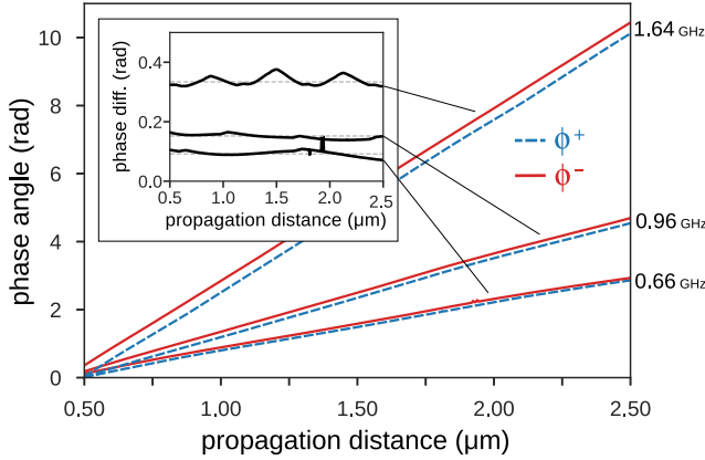
Figure 4. Spin-wave phase profiles \phi(x) along the domain wall for DW^- (solid lines) and DW^+ (dashed lines) for three distinct frequencies. Albeit an absolute and constant phase difference (shown in the inset) 1 , the spatial change in phase (slope of each profile) giving the wave-vector magnitude k along the domain wall is identical for the (-) and (+) propagation directions.
