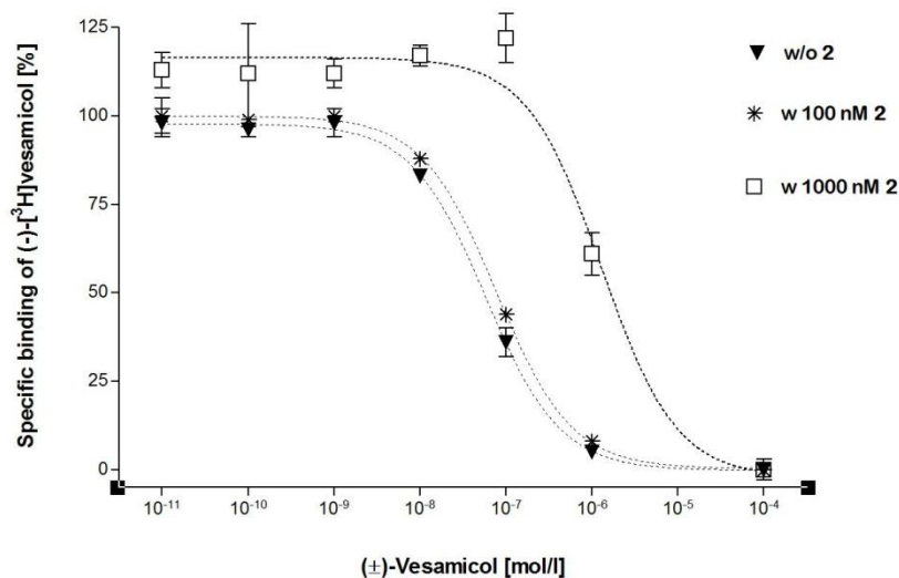
Figure 3. Representation of binding data as non-linearized inhibition curves (one out of three experiments; n=3 per data point).
