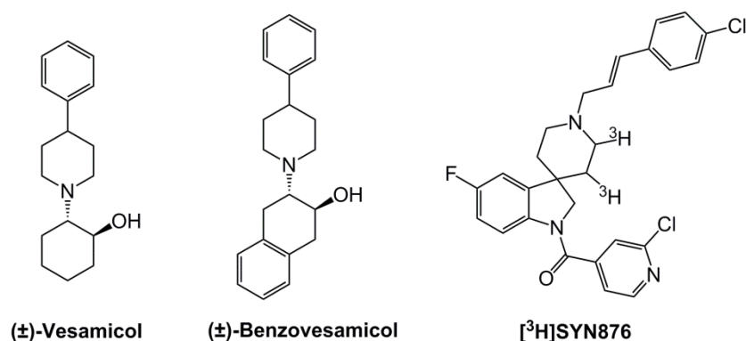
Figure 1. Known VACHT ligands vesamicol, benzovesamicol and spiroindoline [ 3 H]SYN876 as potential lead compounds in the development of VACHT PET radiotracers
