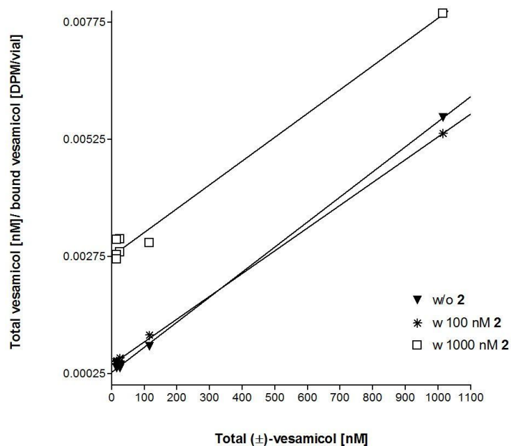
Figure 4. Representation of binding data after Hanes-Woolf linearization.
