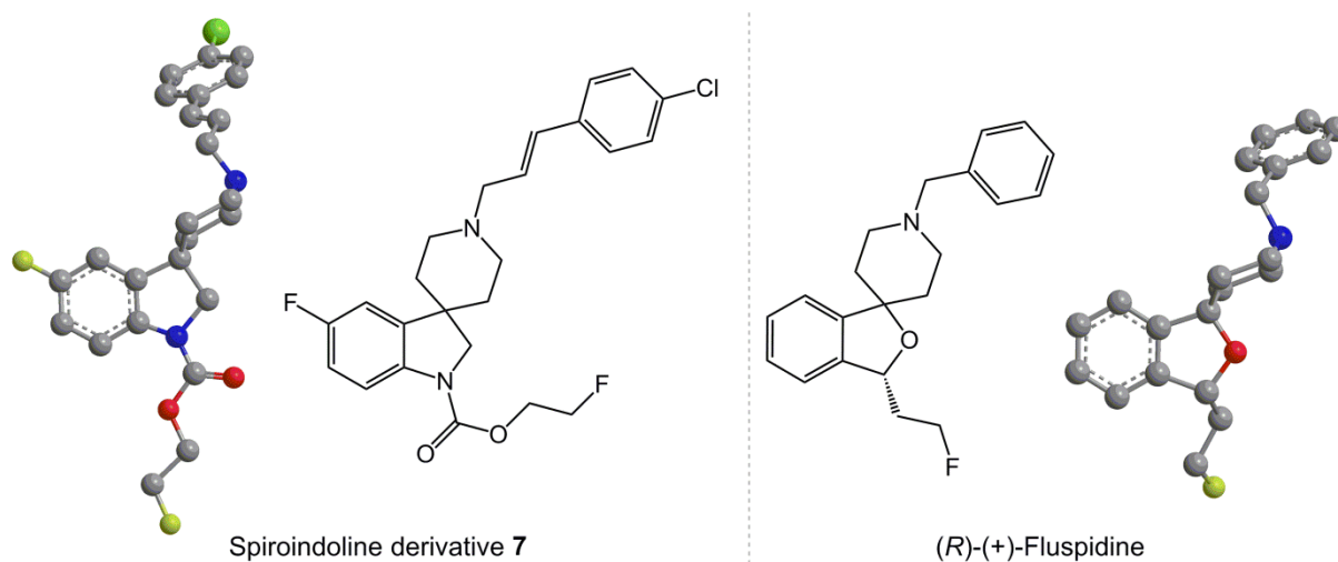
Figure 2. Three-dimensional a molecular structures of compound 7 and the \sigma_1 receptor specific ligand ( R )-(+)-fluspidine; a The 3D-structures were generated with Chem3D Version 16.0 by using MM2 energy minimization.
