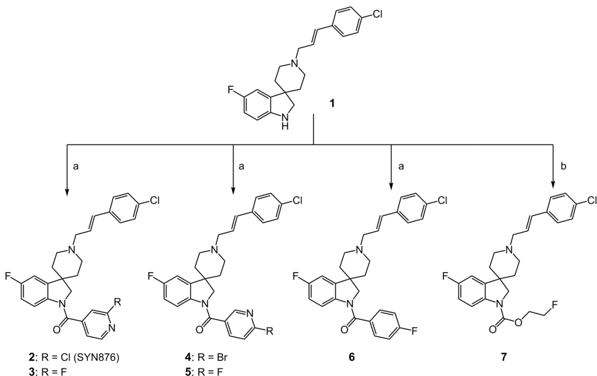
Scheme 1. Reagents and conditions: a) BOP ((benzotriazol-1-yloxy)tris(dimethylamino)phosphonium hexafluorophosphate), TEA (triethylamine), 2-chloroisonicotinic acid for 2 , 2-fluoroisonicotinic acid for 3 , 6-bromonicotinic acid for 4 , 6-fluoronicotinic acid for 5 and 4-fluorobenzoic acid for 6 , CH 2 Cl 2 , rt, 24 h; b) K 2 CO 3 , DMF, 2-fluoroethyl methanesulfonate, 90 °C, 19 h.
