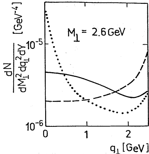
Figure 1: The transverse momentum dependence of the dilepton spectrum from free-streaming parton matter at M_{\perp} = 2.6 GeV according to eq. (6) (full, dotted, dashed lines for (a), (b), (c), respectively).
