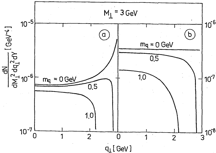
Figure 3: The q_{\perp} dependence of the dilepton spectrum for an initially thermalized quark-gluon plasma with finite quark masses; (a) subsequent free-stream evolution, (b) local thermalization is kept during the subsequent evolution. Initial values are as in Fig. 1 for (a), and T_0 = 333 MeV, \tau_0 = 1 fm/c [24] for (b). When using T_0 = 536 MeV, \tau_0 = .13 fm/c [15] in (b) the curves are shifted up by a factor 1.5.
