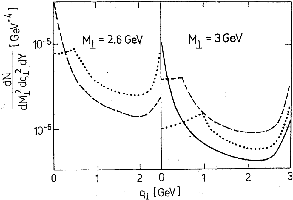
Figure 2: Transverse momentum dependence of dilepton spectrum according to eq. (6b) for M_{\perp} = 2.6 (left panel) and 3 (right panel) GeV, and p_{\perp}^* = 1, 1.25 and 1.45 GeV (dotted, dashed, and full lines).
