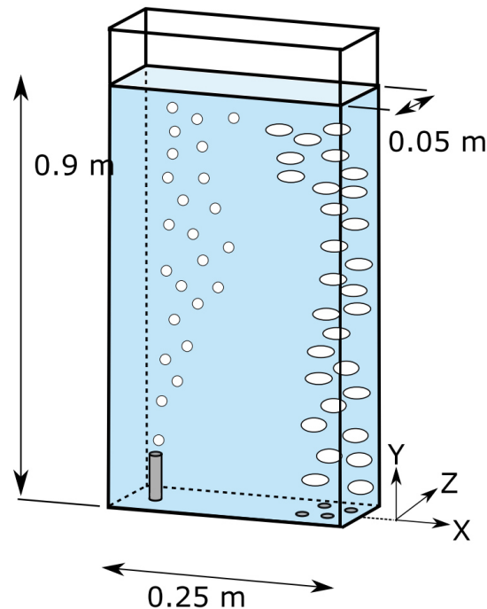
Figure 1 Experimental setup
