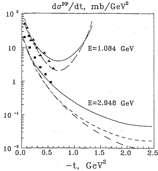
FIG. 1. Elastic \Delta -production cross section for the pp \rightarrow \Delta^{++}n reaction at bombarding energies 1.084 and 2.948 GeV. Experimental data at 1.084 (triangles) are taken from Ref. 17 , while data at 2.948 GeV (squares) are from Ref. 18 . Solid lines correspond to calculations with T -matrix (10) and \Lambda_{NN\pi} = \Lambda_{N\Delta\pi} = 0.7 GeV. Curves representing calculations at 2.948 GeV exploit the T -matrix from Ref. 19 with \Lambda_{NN\pi} = \Lambda_{N\Delta\pi} = 0.545 GeV (long dashes) the T -matrix (10) with \Lambda_{NN\pi} = \Lambda_{N\Delta\pi} = 0.545 GeV (dashes). At 1.084 GeV both latter curves practically coincide (long long dashes).
