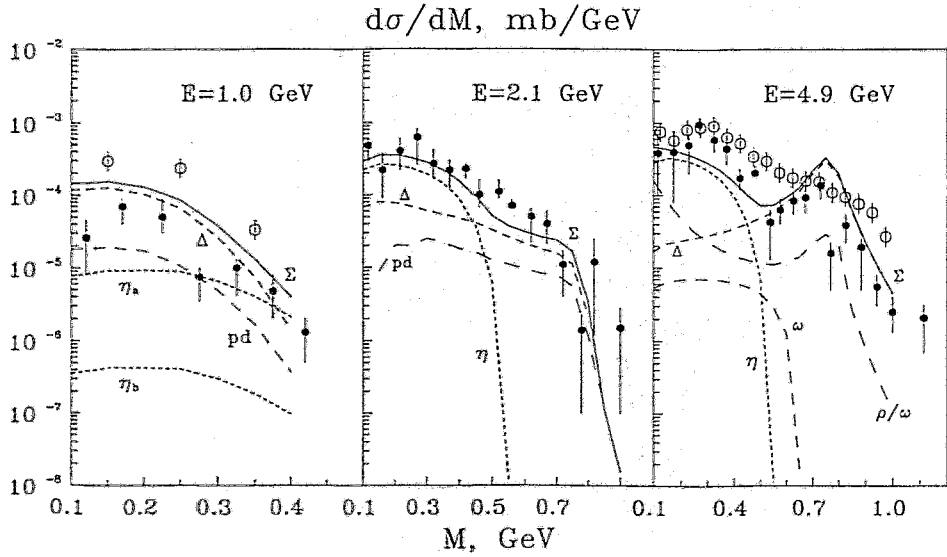
FIG. 5. Dielectron invariant mass spectra for the pN -collision at E = 1.0, 2.1, 4.9 GeV calculated with the DLS filter. Notations for the curves are the same as in Fig. 4. Experimental data for p^9Be collisions, scaled by the factor A^{-2/3} , are taken from Ref. 3 (solid circles). Open circles at 1 GeV represent the product of calculated dielectron yield in pp collisions times the ratio of the pd to pp dielectron production (see the text). Open circles at 4.9 GeV are the experimental data taken from Refs. 2 .
