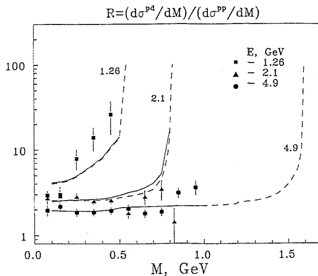
FIG. 6. Ratio of the cross section for pd to pp reactions at E = 1.26, 2.1, 4.9 GeV. The preliminary experimental data are taken from Ref. 2,39 . Dashed and solid lines correspond to the calculation with and without of the DLS filter, respectively.
