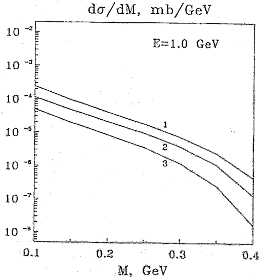
FIG. 3. Contributions of the pn (curve 2) and pp (curve 3) bremsstrahlung to the dielectron production at 1 GeV. The curve 1 represents a contribution of the pn bremsstrahlung calculated within the soft photon approximation [see Eq. (19)].
