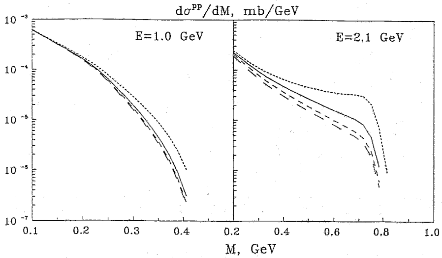
FIG. 2. The Dalitz delta decay contribution to the dielectron production at E = 1 and 2.1 GeV. The results of calculations with the constant production cross section \bar{\sigma}_{\Delta}(s, M_{\Delta}) in Eq. (1) are represented by the short-dashed curve, while other curves correspond to different \Delta production T -matrices. Notation is the same as in Fig. 1.
