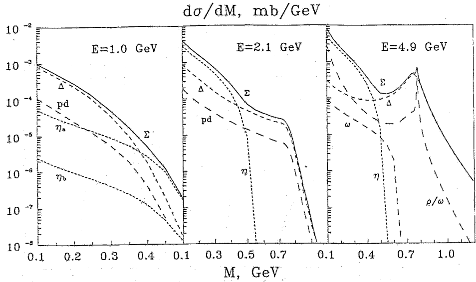
FIG. 4. Dielectron invariant mass spectra for the pN -collision ( pN = pd/2 ) at E = 1.0, 2.1, 4.9 GeV calculated without the DLS filter. The “ pd ” labels bremsstrahlung, “ \eta ”, “ \Delta ” and “ \omega ” denote the corresponding Dalitz decay contributions, “ \rho/\omega ” is the direct rho-omega decay, “ \Sigma ” is the sum of all contributions. The line \eta_b at 1 GeV represents the subthreshold \eta decay contribution with taking into account the internal nucleon motion in a deuteron; the line \eta_a shows calculations with the two-nucleon short-range correlation.
