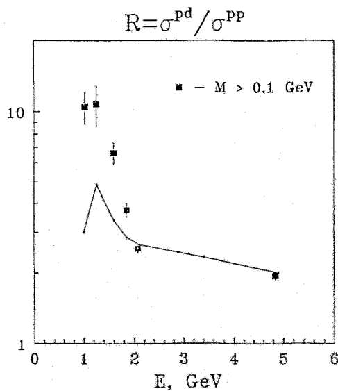
FIG. 7. Ratio of the integrated cross section for pd to pp reactions as function of the initial energy. Solid line corresponds to the calculation with the DLS filter. The preliminary experimental data are taken from Refs. 2,39 .
