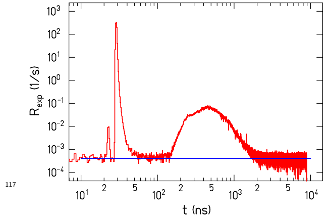
Fig. 2. Dead-time corrected time-of-flight spectrum with Au sample from a subset of the data taken ( t_{\text{real}} = 37200 s). PMT after-pulses are suppressed as described in the text. A narrow condition on the time-difference of the PMT signals is used to suppress e.g. double hits. The first peak at 22 ns is due to double hits in the scintillator. The bremsstrahlung peak is located at 28.4 ns, its width is 1.25 ns (FWHM). The neutron time-of-flight range is from about 150 to 2500 ns. The blue line is the result of a fit of a constant time-independent background rate. The bin size of the spectrum is 0.5 ns.
