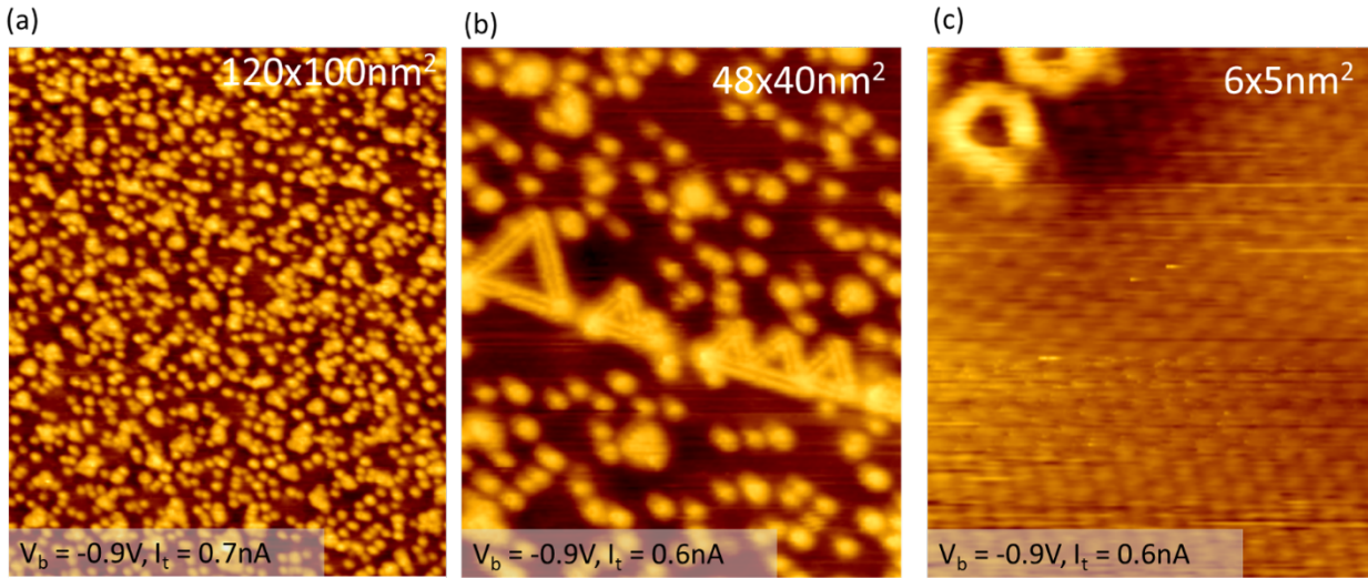
Figure 8: STM of 0.3% of a titanium ML deposited on \text{MoTe}_2 at 350^\circ\text{C} (a) Large scale image showing single protrusions together with some small triangular MTBs. (b) some larger triangular MTB-loops are occasionally observed that appear to be aligned and thus suggesting that some pre-existing line defect in the substrate may assist their formation. (c) Zoom-in on bright protrusions shows a similar ring structure as has been observed for single Mo-interstitial sites, suggesting that every protrusion is due to a Ti-interstitial.
