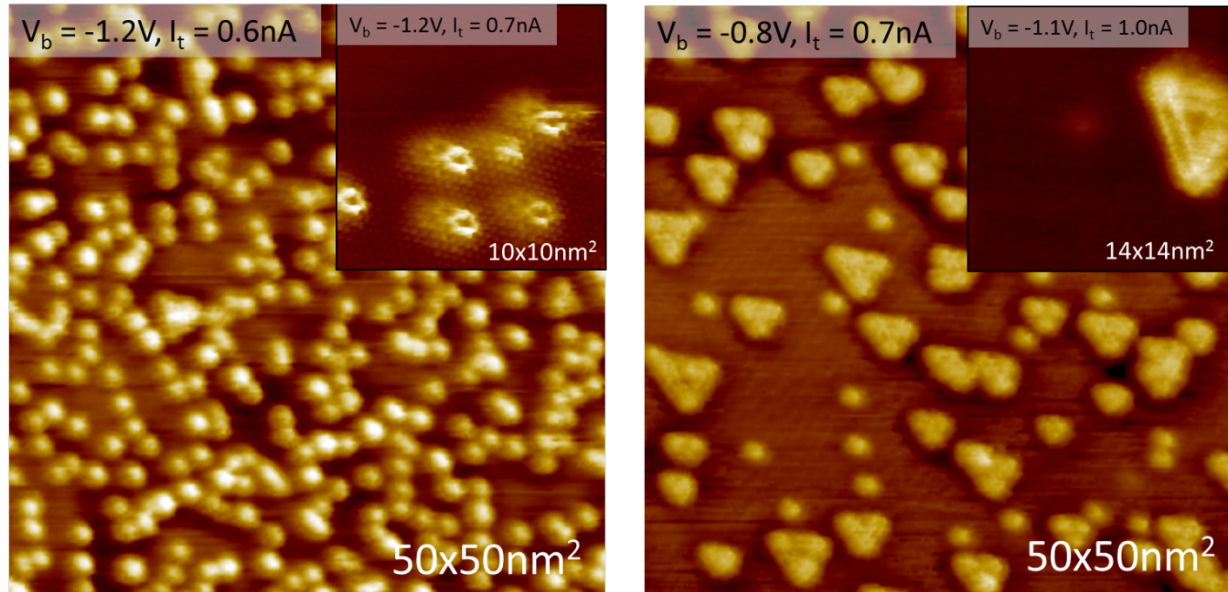
Figure 3. STM studies of MoTe 2 surfaces with Mo deposited at room temperature and subsequent annealing. (a) Large scale STM images of MoTe 2 after Mo deposition at room temperature. The inset shows the structure of individual Mo-induced point defects (likely Mo-interstitials). (b) Large scale STM images of MoTe 2 after annealing at 250°C. Annealing at such temperature converts the point defect into MTB-loops clearly resolved in the inset.
