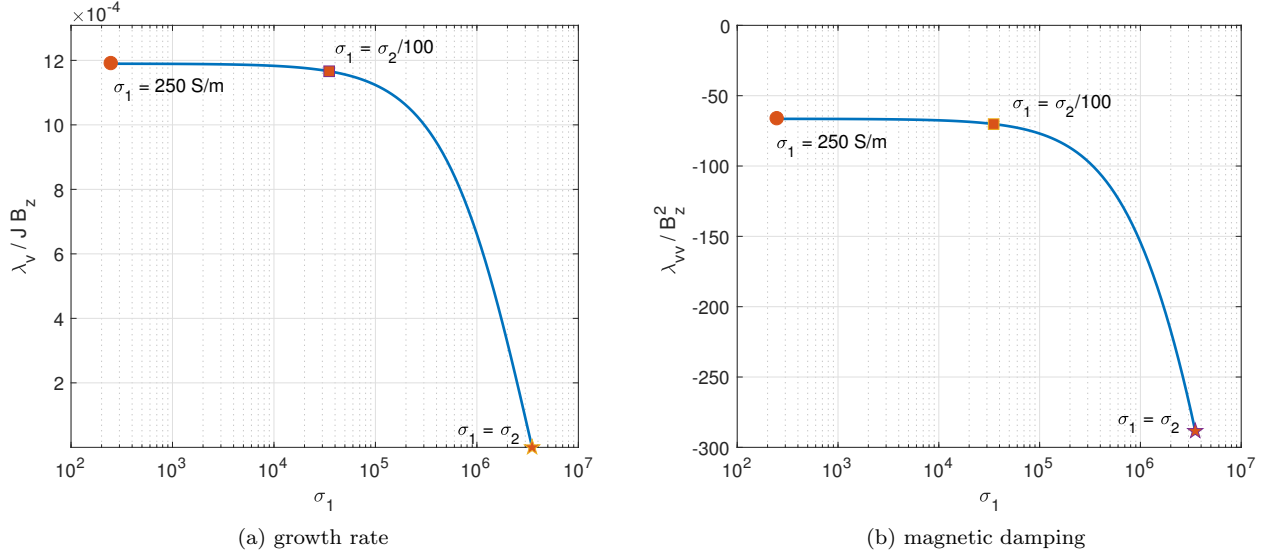
FIG. 6. Variation of the relative growth rate \lambda_v/JB_z (panel (a)) and magnetic damping term \lambda_{vv}/B_z^2 (panel (b)) when \sigma_1 is artificially increased. From \sigma_1 = 250 S/m to \sigma_1 = \sigma_2/100 there is only a weak modification of the growth rate and magnetic damping. This suggests that, in direct numerical simulations, one can significantly relax the conductivity jump, without modifying the linear instability characteristics. At \sigma_1 = \sigma_2 , the instability vanishes: a strong difference in conductivity is essential for the metal pad roll instability.
