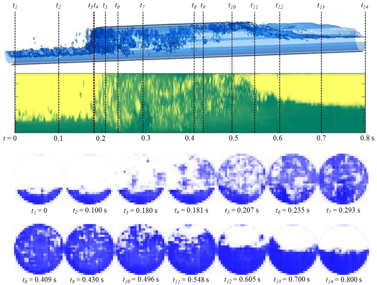
Fig. 10. WMS Data Visualization of a Slug Body ( \theta = 10^\circ ; v_{SL} = 0.005 m/s; v_{Sg} = 2.6 m/s; v_T = 3.9 m/s) (Top: iso-surface created by Tecplot™ 360; Middle: liquid holdup evolution at pipe center; Bottom: liquid phase distribution at different time)
