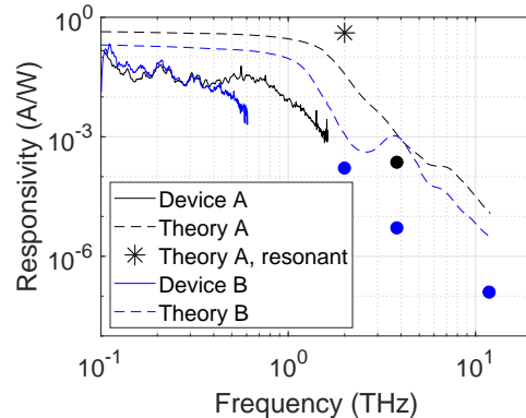
Fig. 4. Measured and calculated responsivity of device A and B. The peak in the theoretical responsivity for device B between 3 and 4 THz arises from a resonance in the antenna simulations which is not observed in the experiment. The measurements are referenced by the total (peak) power of the respective sources and are only corrected for the frequency dependent polarization mismatch and the reflection of the silicon lens. With a resonant antenna the responsivity is expected to increase by an order of magnitude at 2 THz (star).
