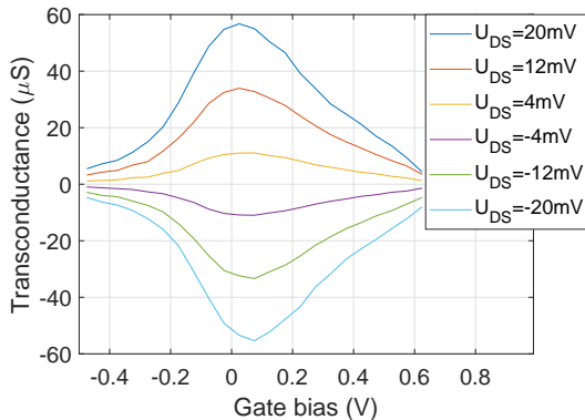
Fig. 3. DC transconductance of sample A, showing a pronounced extremum close to 0 V gate bias, qualifying the transistor for zero-bias operation.
