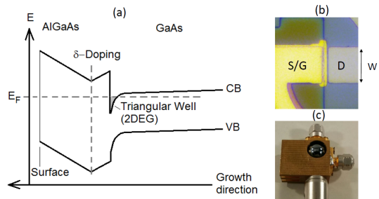
Fig. 1. (a) HEMT band structure of the FET. (b) Micrograph of the fabricated device A. (c) Silicon-lens integrated housing
