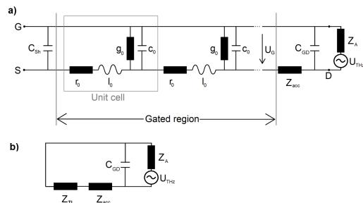
Fig. 2. (a) Detailed equivalent circuit of the FET. (b) Lumped element representation.
