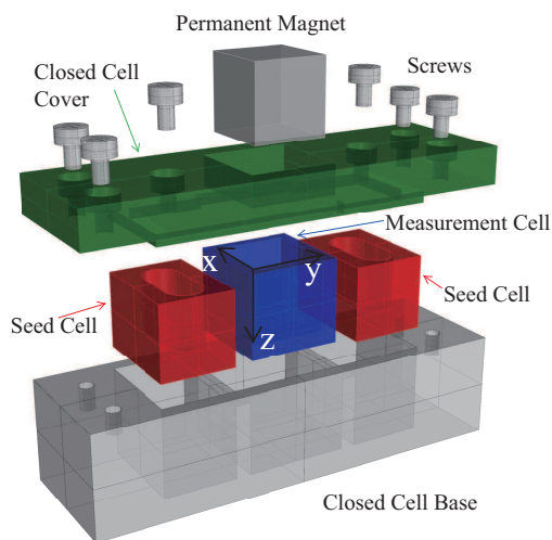
Figure 1: Schematic diagram of the setup consisting of an outer plexiglass cell (gray and green parts) which provides a closed system for mass, a high-quality optical quartz glass measurement cell, two seed cells made of Teflon and the NdFeB permanent magnet.
