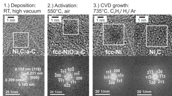
High-resolution TEM micrographs and corresponding FFTs reveal the phase transformations of Ni-rich nanoparticles of C:Ni nanocomposite templates during the steps of the CVD synthesis of diameter-controlled SWCNTs.
