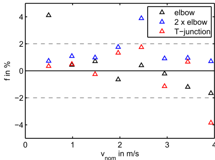
Figure 7. Measured relative deviation from nominal velocity.
