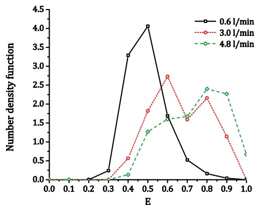
Figure 11 Number density distribution of the aspect ratio in the range 0.75 \leq E_o \leq 1.25
