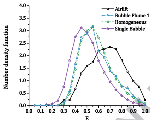
Figure 13 The aspect ratio distribution in the range 1 < Eo < 2
