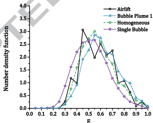
Figure 14 The aspect ratio distribution in the range 2 < Eo < 3
