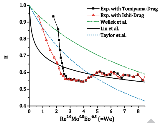
Figure 16 Aspect ratios as a function of the Weber number.
