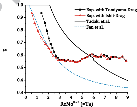
Figure 17 Aspect ratios as a function of the Tadaki number.
