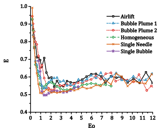
Figure 12 Aspect ratios for different experiments.
