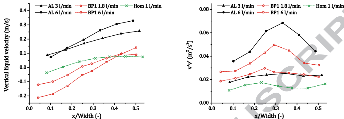
Figure 4 Measured vertical liquid velocity ( v ) and the normal Reynolds stress tensor component v'v' for different setups (see Table 1 for abbreviations) and flow rates at y = 0.6 m. For the airlift reactor, only the results in the riser are shown. Due to symmetry, only one-half of the column is shown.
