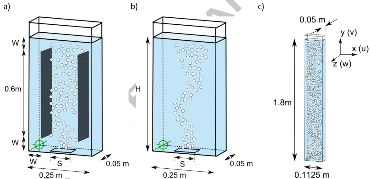
Figure 3 Experimental setup of the airlift a), bubble plume 1 and 2 as well as single needle experiments b), and the homogeneously aerated bubble column c)
