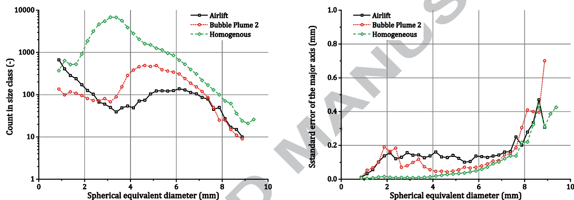
Figure 7 The bubble count (left) and the standard error ( = \frac{1}{\sqrt{N}} \sigma ) of the major axis (right) for the Airlift, Bubble Plume 2, and Homogeneous experiment with respect of 0.25 mm bubble size classes.
