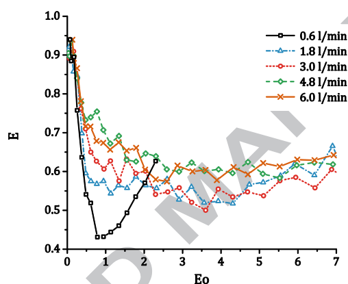
Figure 10 Aspect ratios for the bubble plume experiment BP1 at different gas flow rates.
