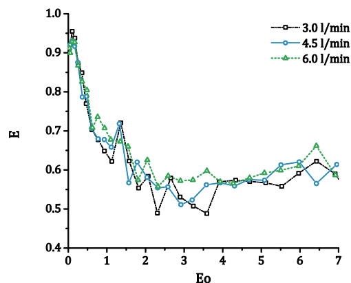
Figure 9 Aspect ratio at different gas flow rates in the riser of the airlift reactor.
