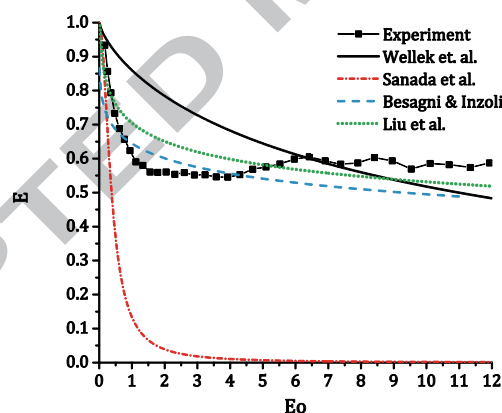
Figure 15 Aspect ratios as a function of the Eötvös number.
