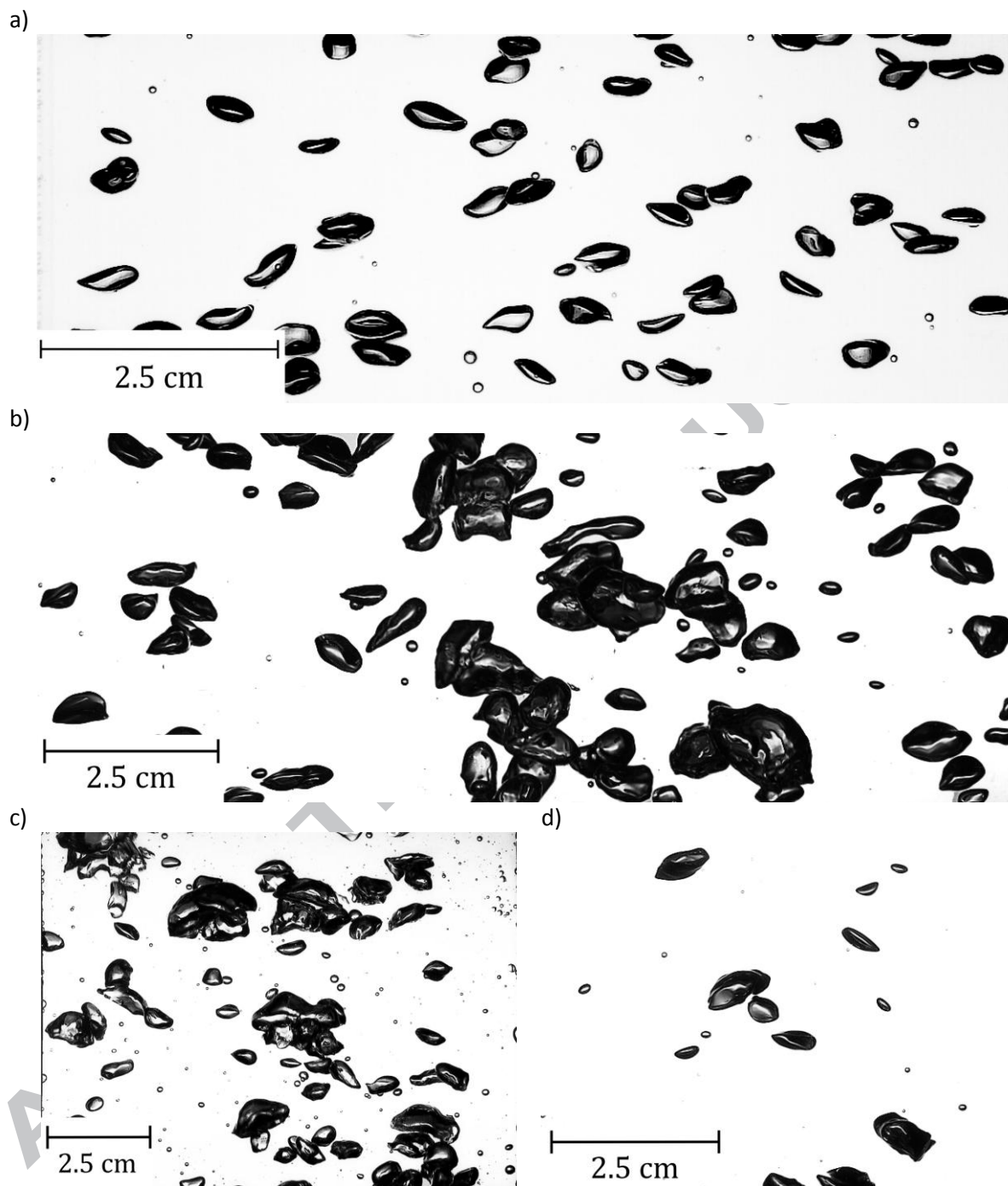
Figure 6 Pictures used for bubble size evaluation a) homogenous bubble column with 0.3 mm needles b) bubble plume 2 with 0.6 mm needles and a gas flow rate of 4.0 l/min c) airlift reactor at a gas flow rate of 4.5 l/min and d) single needle experiment with 0.6 mm needles and 0.5 l/min.
