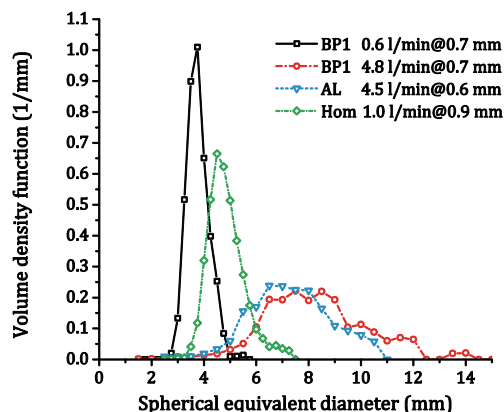
Figure 8 Bubble size distribution for different gas flow rates and needle sizes.
