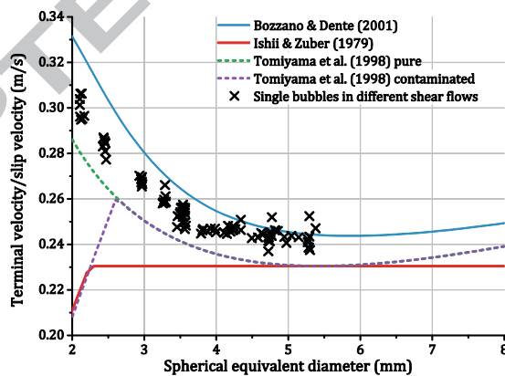
Figure 5 Measured slip velocity compared to different terminal velocity models
