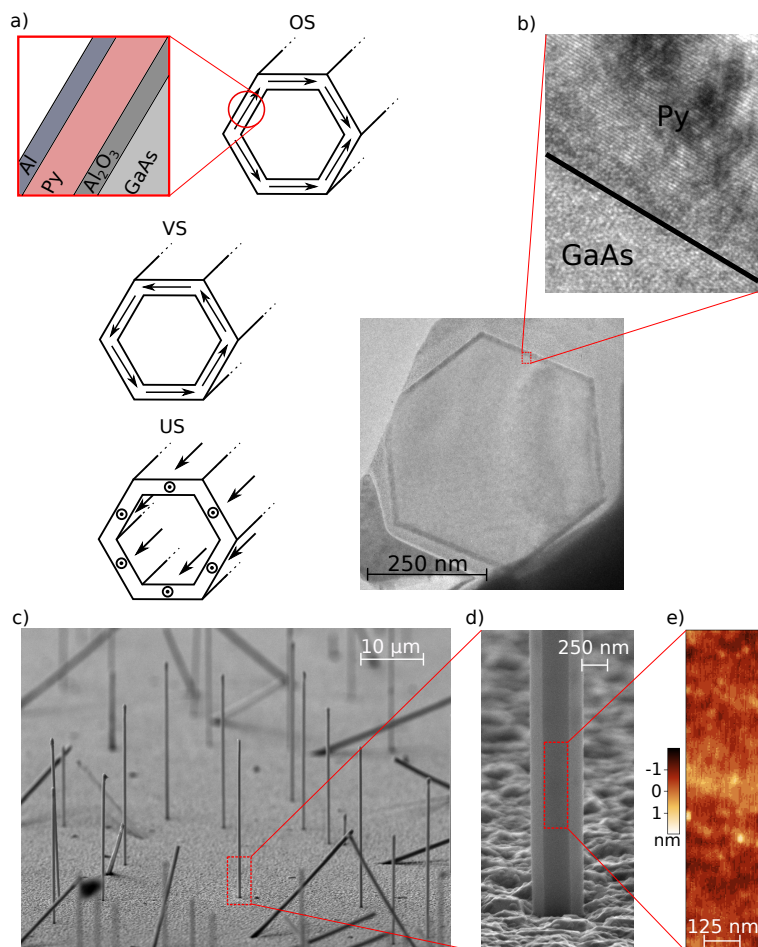
Figure 1: a) Illustration of different states found in magnetic NTs and sketch of the layers deposited on the GaAs core. The thicknesses of the different layers for the samples are specified in Table 1. While the vortex state (VS) and the uniform state (US) may appear as magnetic ground states, the onion state (OS) is metastable and can only be entered after the application of an external magnetic field. b) Cross sectional TEM image of sample s1. The inset shows an enlargement of the border between GaAs and Py. The crystalline structure of Py can be identified. c) SEM image of the free standing, low density NTs which are individually selected for the experiments. d) Hexagonally shaped NTs exhibiting a very smooth surface after metal layer deposition. e) AFM images of the facets reveals a root mean squared roughness of R_{\text{rms}} = 0.4 nm.
