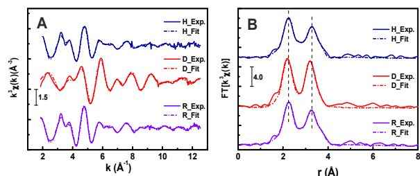
Figure 2. A). Ag K-edge of k^3 -weighted EXAFS function and B). Corresponding phase corrected Fourier Transfer (FT) best fits of the sample in hydrated (H), dehydrated (D), and rehydrated (R) states. The experimental (Exp.) and fitted data are indicated with solid and broken lines to visualize the fitting quality.
