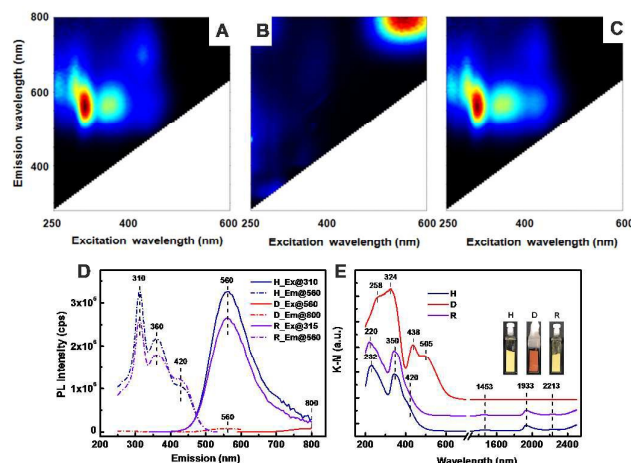
Figure 1. 2D excitation-emission plots of the sample in A) Hydrated, B) Dehydrated, C) Rehydrated states. D) Luminescent PL intensity of the sample at different excitation (Ex.) and emission (Em.) maxima in hydrated (H), dehydrated (D) and rehydrated (R) states. E) Diffuse reflectance UV-Visible-NIR spectra of the samples, the inset shows the actual colours of the sample in its different hydration states.
