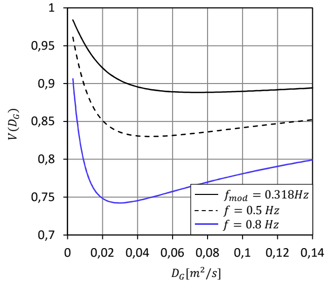
Figure 11: Amplitude damping V(D_G) for increasing modulation frequencies for measured u_s = 0.38 m/s for measurements between x_1 = 0.15 m (ref) and x_2 = 0.23 m.
