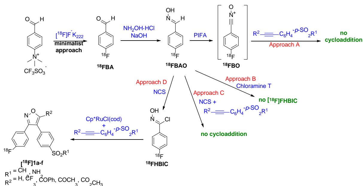
Scheme 2. Approaches for ^{18}\text{F} FHBIC synthesis and Ru-promoted 1,3-dipolar cycloaddition
