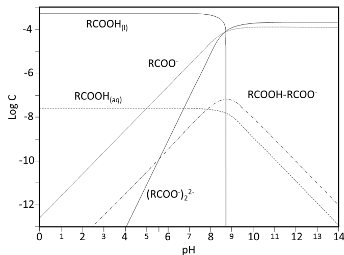
30 31 32 33 34 35 36 37 38 39 40 41 42 43 44 45 46 47 Figure 11: Species distribution diagram of sodium oleate at a concentration of 5.26 \times 10^{-4} mol/l modified from [39] (in the 48 flotation testwork, concentration of sodium oleate at the beginning of the tests was of 2.65 \times 10^{-4} mol/l)
