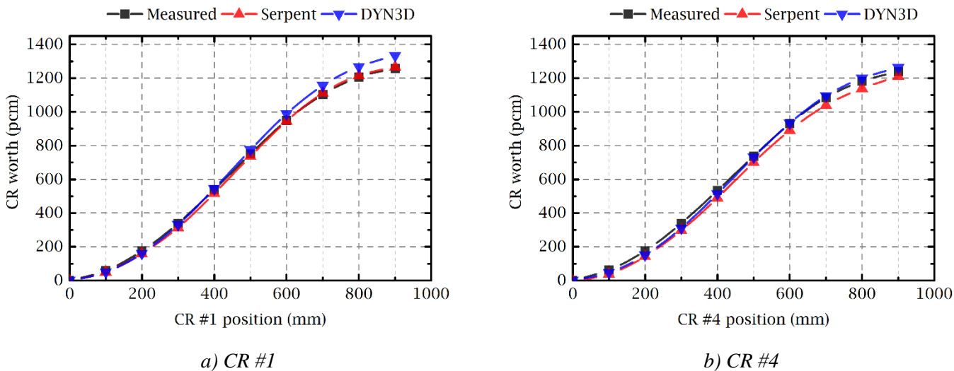
Fig. 8. Comparison of control rod S-curves.
