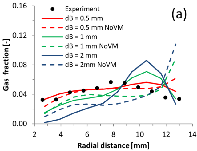
Fig. 8. Radial profiles of gas fraction at measurement plane H1 for the inlet gas volume fraction \varepsilon_{in} = 5\% . (a) Comparison of simulations with and without virtual mass force model. (b) Comparison of simulations assuming mono-disperse and bimodal bubble sizes.
