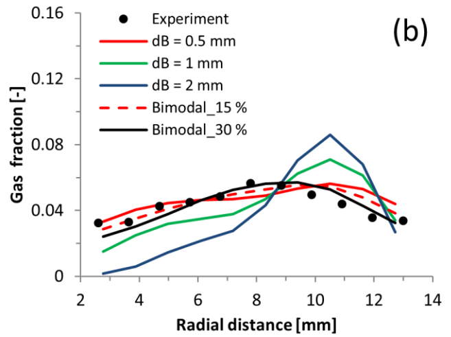
Fig. 8. Radial profiles of gas fraction at measurement plane H1 for the inlet gas volume fraction \varepsilon_{in} = 5\% . (a) Comparison of simulations with and without virtual mass force model. (b) Comparison of simulations assuming mono-disperse and bimodal bubble sizes.
