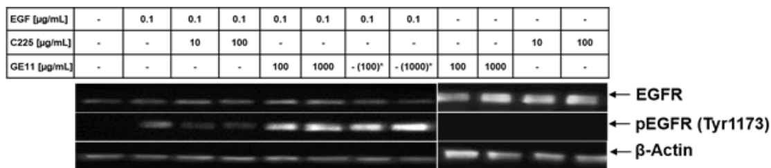
Fig. 8 Immunologic detection of EGFR (Y1173) phosphorylation levels, EGFR and \beta -actin upon treatment with EGF in combination with C225 or GE11. Vehicle control was PBS + 5% DMSO. Western blot analysis (lower part) was performed for phosphorylated EGFR (pEGFR, Y1173), total EGFR, and \beta -actin by incubation with respective primary antibodies followed by incubation with HRP-coupled secondary antibodies and chemiluminescence detection. The different intensity of \beta -actin and EGFR bands occurred since the blot of the last 4 lanes on the right side was obtained from a separated immunoblotting assay. The data represent only qualitative estimation. Similar results were obtained in three independent experiments
