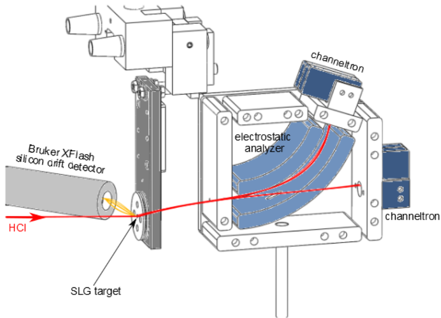
Figure 1: Sketch of the experimental setup. The collimated ion beam is passing the sample, mounted on the rotatable target holder, before it enters the electrostatic analyzer and hits one of the channeltrons.
