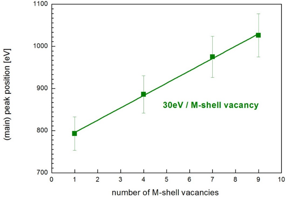
Figure 5: Linear increase of M-shell X-ray emission energy for increasing incident \text{Xe}^{q+} charge state. The main peak ( 4f \rightarrow 3d ) energy shifts about 30 eV towards higher energies for every additional M-shell vacancy.
