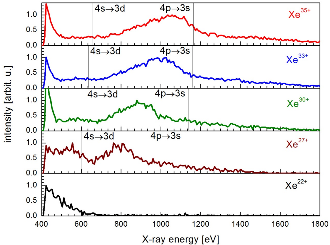
Figure 4: X-ray emission resulting from filling of M-shell vacancies (main peak) and high energy tail of N-shell filling (above noise and below 700 eV) for Xe ions at 100 keV with 0, 1, 4, 7 and 9 M-shell holes. High energy tail of main peak due to electron transitions from n > 4 levels into M-shell vacancies.
