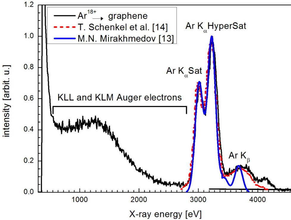
Figure 3: X-ray, KLL and KLM Auger electron emission recorded for bare Ar^{18+} ion impact on SLG. The measured X-ray spectrum (black solid line) is compared with tabulated radiative transition amplitudes for Ar^{18+} impact on metal surfaces [13] (blue curve) and measured data for Ar^{18+} impact on Be [14] (red broken curve).
