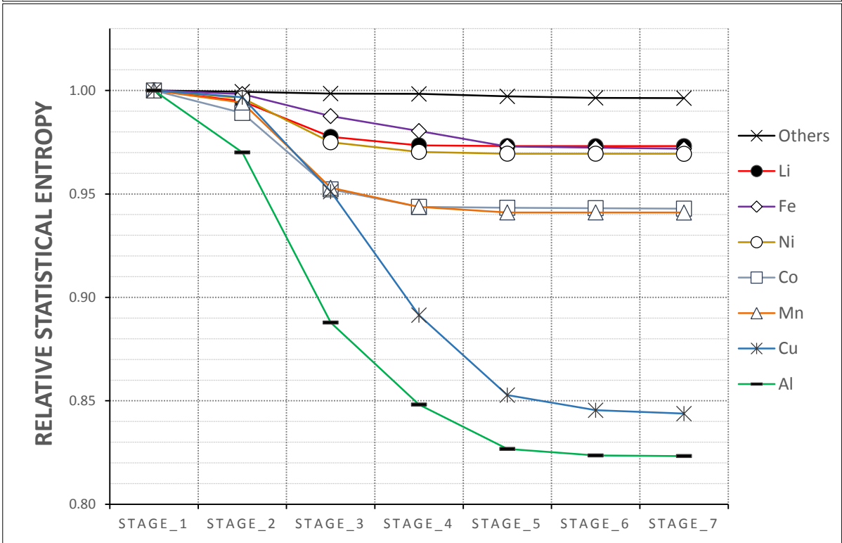
Figure 6 Evolution of: total RSE and Exergy (top), and, RSE per element (bottom) for the original sieving system.
