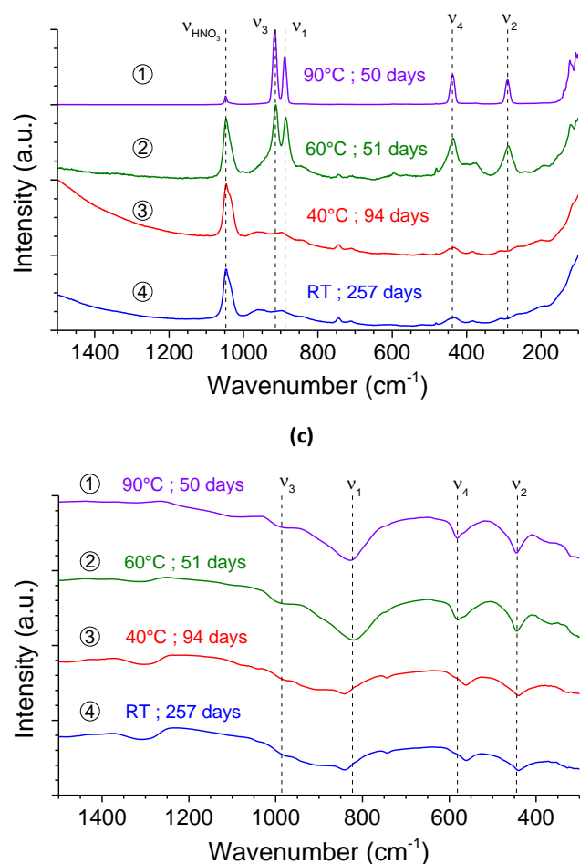
Figure 1. PXRD patterns (a), Raman (b) and infrared spectra (c) obtained for samples prepared with starting silicate and thorium(IV) concentrations of 0.21 \text{ mol}\cdot\text{L}^{-1} in nitric reactive media at initial pH = 3 at 90°C for 50 days (1), 60°C for 51 days (2), 40°C for 94 days (3) and at room temperature for 257 days (4). Characteristic XRD lines of \text{ThO}_2 and \text{ThSiO}_4 were extracted from references 40 and 3 , respectively.
