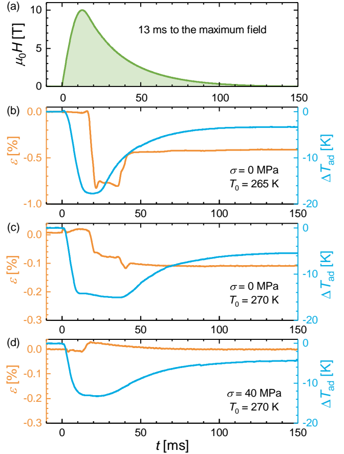
FIG. 4. (a) Time dependence of the magnetic field in the coil. The rise time of the field accounts for 13 ms. (b) - (d) The strain \varepsilon of the sample during the experiment is shown on the left and the adiabatic temperature change \Delta T_{\text{ad}} on the right axes.
