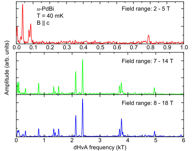
FIG. 2. dHvA frequency spectra obtained from the torque data shown in Fig. 1 for different field ranges. Note the different scaling of the frequency axes between the top and the two bottom panels.
