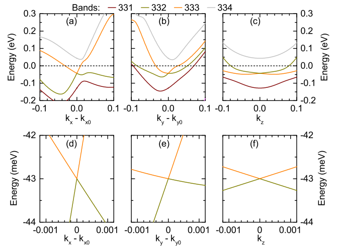
FIG. 6. Band structure of \alpha -PdBi in the vicinity of the Weyl node at \mathbf{k}_0 = (k_{x0}, k_{y0}, k_{z0}) = (0.399706, 0.056504, 0)2\pi/a . The cuts are running parallel to the (a) k_x , (b) k_y , and (c) k_z directions. The band colors are identical to those used in Fig. 5(a). (d), (e), and (f) are zooms into (a), (b), and (c), respectively. In these zoomed images, we used a fine k spacing of steps in the range |\mathbf{k} - \mathbf{k}_0| \leq 10^{-3} in order to show that the crossing is indeed nearly linear in all directions.
