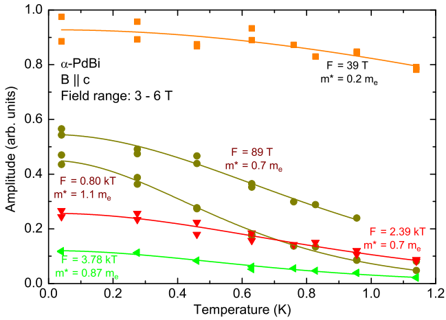
FIG. 3. Effective masses determined by fits of the Lifshitz-Kosevich formula (lines) to the temperature-dependent dHvA oscillation amplitudes (symbols).
