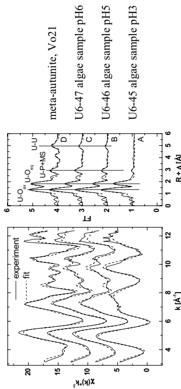
Fig. 1. Raw U L III -edge k 3 -weighted EXAFS spectra (left) and corresponding Fourier transform (right) of the algae samples and meta-autunite at 30 K.
