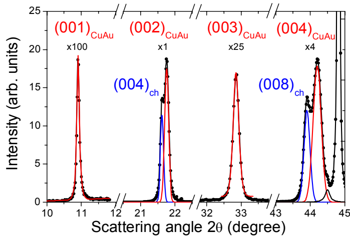
Fig. 3. XRD-spectra of the (00l) in-plane reflections. Mixed Lorentz / Gauß-profiles (solid lines) were fitted to the spectra. The high diffraction intensity around 2\theta = 44.8^\circ is due to the Si-substrate.
