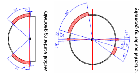
FIG. 1: Improved sputter deposition chamber with larger window openings made of Beryllium installed into the 6-circle ROBL diffractometer.
