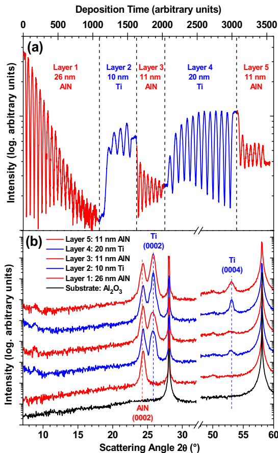
Fig. 5. (a) shows in situ time-resolved x-ray reflectivity taken during sequential deposition steps of epitaxial AlN and Ti on Al_2O_3(0001) and (b) shows the corresponding XRD patterns recorded after each deposition step.
