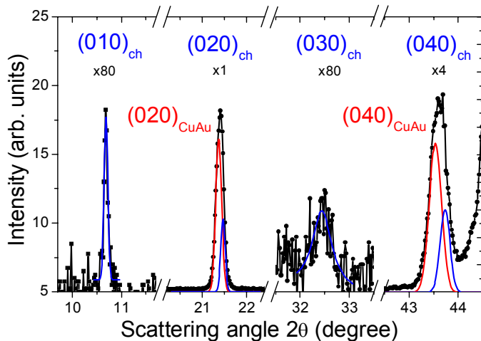
Fig. 4. XRD-spectra of the (0k0) out-of-plane reflections as measured in transmission geometry.
