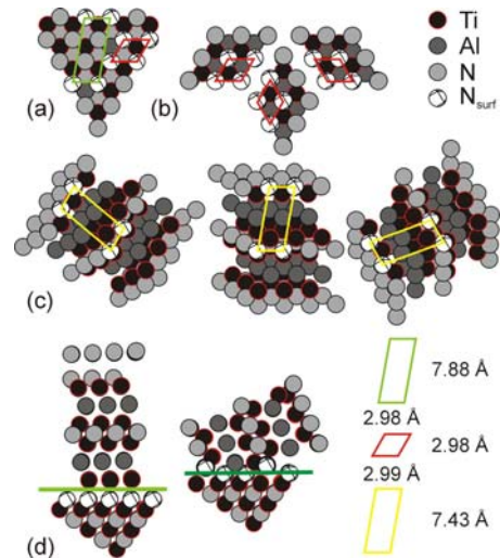
Fig. 4. Atomic illustration of (Ti 0.63 Al 0.37 )N and Ti 2 AlN planes and directions (a) shows the (Ti 0.63 Al 0.37 )N(111) surface and (b) the three different Ti 2 AlN{0001} orientations along (Ti 0.63 Al 0.37 )N<110>. (c) shows the threefold orientation for the Ti 2 AlN{1012} planes. (d) shows cross-sectional views of the Ti 2 AlN/(Ti 0.63 Al 0.37 )N interface for basal-plane and non basal-plane growth.
