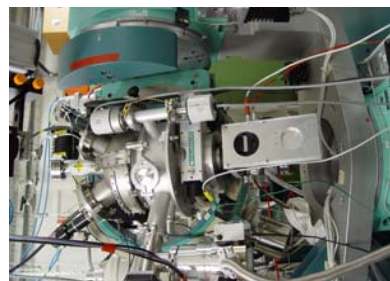
FIG. 1: Improved sputter deposition chamber with larger window openings made of Beryllium installed into the 6-circle ROBL diffractometer.
