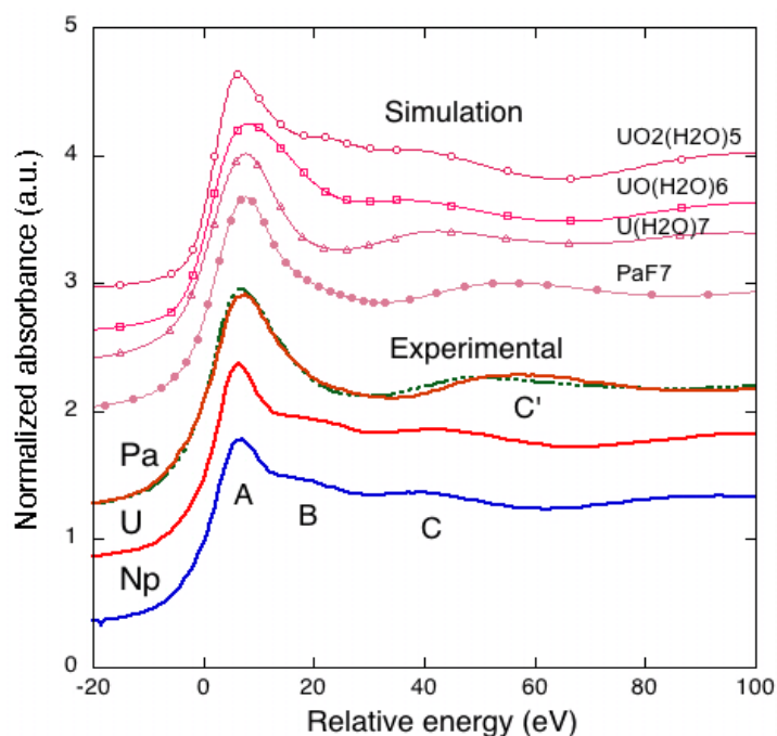
Fig. 2. Experimental and simulated L_{III} edge XANES spectra of Pa(V), U(VI) and Np(V) species. All spectra are normalized and shifted with respect to the inflexion point energy.
