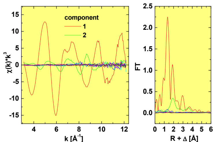
Fig. 2. Abstract spectra of components 1-10 and corresponding Fourier transforms.
