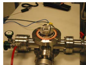
In-house designed chamber with hemispherical Be-window (i.e. 2π x-ray access for GIXS) for moderate annealing temperatures (< 900°C).
