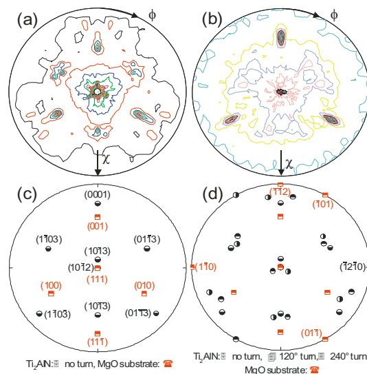
Fig. 2. Pole figures of Ti 2 AlN grown onto MgO(111), nominally measured on (a) Ti 2 AlN(1073) and (b) Ti 2 AlN(0002). The stereographic projection (c) shows the theoretical poles of Ti 2 AlN{1073}, {1072}, {0001}, {2110} and MgO{111}, {110}, {112}. (d): The experimental pole figures in (a) and (b) can be obtained by turning (c) for 120°, as indicated by the symbols.
