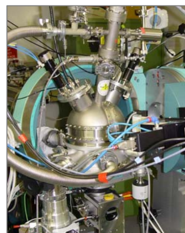
Two magnetron sputter deposition chamber with mounted ion irradiation gun (top).
