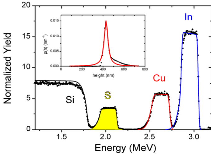
Fig. 2. RBS-spectrum of an epitaxial CIS-thin-film on Si(001). The contributions of the individual elements to the spectrum are indicated. The inset shows the normalized height distribution of the sample as derived from the RBS-spectrum. The spectrum was recorded with an incident \alpha -energy of 3.5 MeV.
