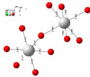
Fig. 4. Local structure around the noncoordinated uranium atom in BaU 2 O 7 .
