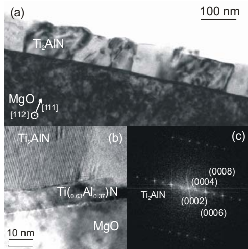
Fig. 3. XTEM micrographs of Ti 2 AlN grown on MgO(111) along the MgO[112] zone axis. (a) shows the film morphology consisting of large crystal regions. (b) shows a high resolution micrograph at the interface with the typical MAX phase 2-1-1 layered structure. It is made up by the (000) planes as confirmed from the d-spacing calculation by Fast Fourier Transformation in (c).
