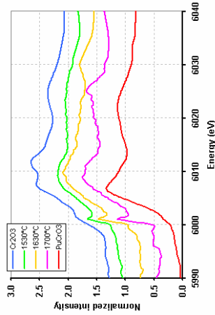
Figure 1 : XANES spectra at the chromium (5.989 keV) K edge.
