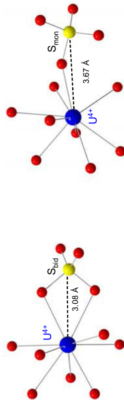
FIGURE 2. Structure of \text{U}(\text{SO}_4)_{\text{bid}}(\text{H}_2\text{O})_7^{2+} and \text{U}(\text{SO}_4)_{\text{mon}}(\text{H}_2\text{O})_8^{2+} complexes.
