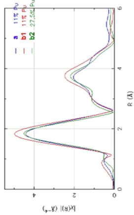
Figure 2 : Fourier transforms of the plutonium L III edge EXAFS (k-range: 2 – 10.5 Å -1 ).
