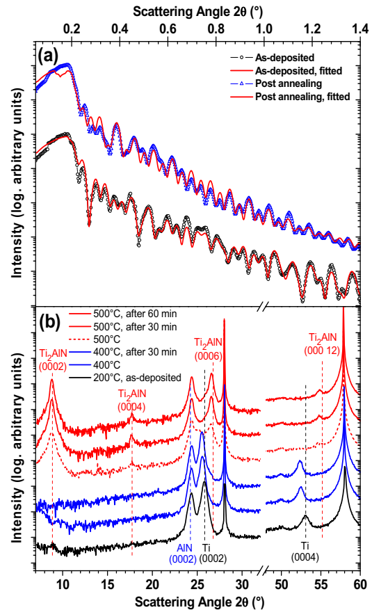
Fig 6. (a) shows experimental and fitted in situ angular resolved x-ray reflectivity of the as-deposited and annealed film, and (b) shows the large angle XRD data recorded every 30 minutes during annealing between 400\text{--}500^\circ C .
