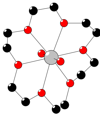
Figure 1: The [UO_2(18\text{-crown-6})]^{2+} cation. 11
