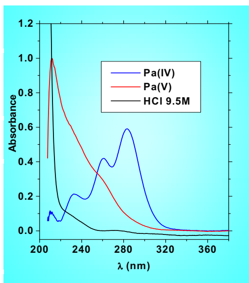
Fig. 1. UV-vis absorption spectra of protactinium (IV) and (V) in concentrated HCl ( C_{Pa} = 9 \times 10^{-3} \text{ M} )
