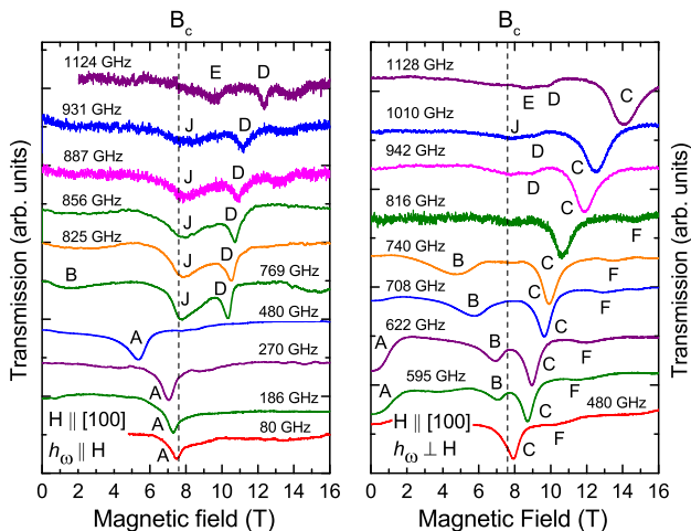
FIG. 6. Examples of polarized ESR spectra in \alpha - \text{RuCl}_3 for h_\omega \parallel H (a) and h_\omega \perp H (b) ( h_\omega is the magnetic component of the THz radiation). H \parallel [100] , T = 1.5 K. The spectra are normalized by the zero-field transmittance background and offset for clarity. The vertical line indicates the critical field as determined in Ref. [9].
