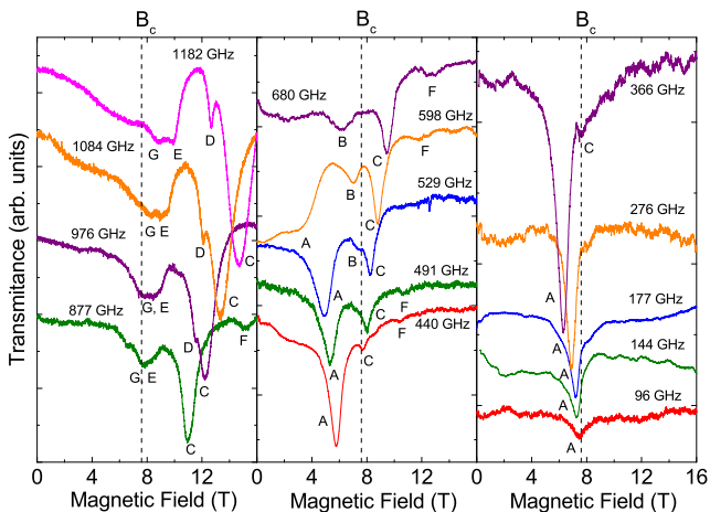
FIG. 3. Examples of unpolarized ESR spectra in \alpha -RuCl 3 for H \parallel [100] at various frequencies; T = 1.5 K. The spectra are normalized by the zero-field transmittance background and offset for clarity. The vertical line indicates the critical field as determined in Ref. [9].
