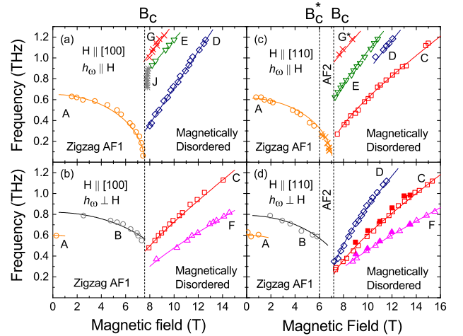
FIG. 2. Frequency-field dependences of magnetic excitations in \alpha -RuCl 3 for H \parallel [100] (a, b) and H \parallel [110] (c, d) ( h_\omega \parallel H (a, c), h_\omega \perp H (b, d), where h_\omega is the magnetic component of the THz radiation; T = 1.5 K). Absorptions denoted by crosses were observed using unpolarized radiation. Solid lines are guides to the eye. The vertical dashed lines indicate critical fields as determined in Ref. [9]. The closed squares and triangles in (d) denote inelastic neutron-scattering data from Ref. [10].
