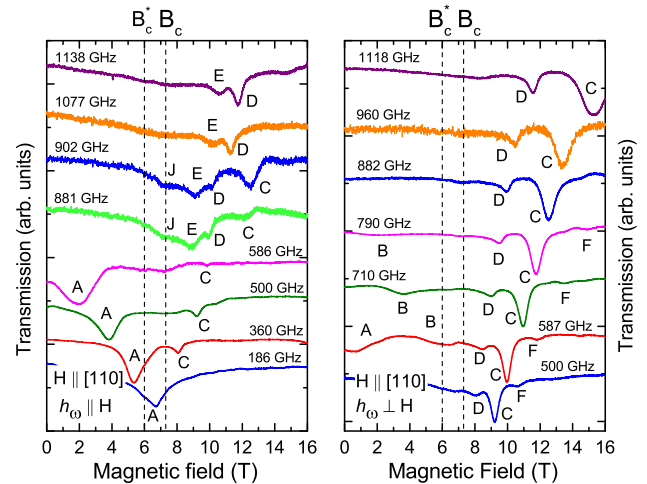
FIG. 7. Examples of polarized ESR spectra in \alpha - \text{RuCl}_3 for h_\omega \parallel H (a) and h_\omega \perp H (b) ( h_\omega is the magnetic component of the THz radiation). H \parallel [110] , T = 1.5 K. The spectra are normalized by the zero-field transmittance background and offset for clarity. The vertical lines indicate the critical fields as determined in Ref. [9].
