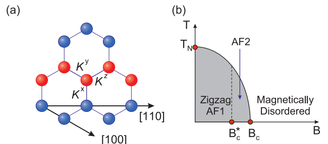
FIG. 1. (a) Schematic view of the honeycomb structure, showing the [100] and [110] axes relative to the Ru–Ru bonds. Ru ions from adjacent zigzag chains are shown by different colors. (b) Schematic temperature-field phase diagram for \alpha -RuCl 3 . AF1 and AF2 correspond to different low-temperature anti-ferromagnetically ordered phases.
