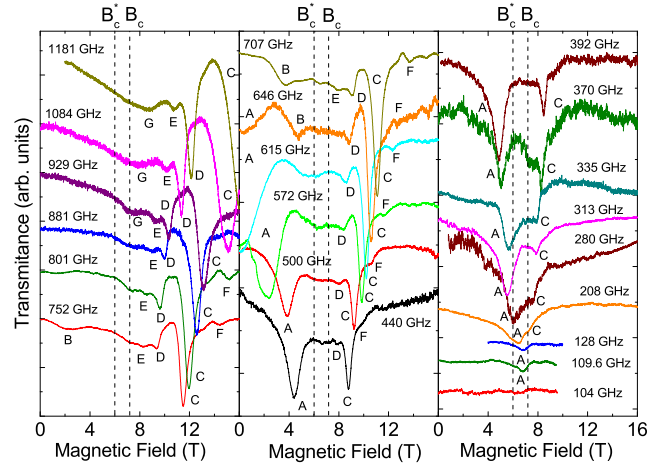
FIG. 4. Examples of unpolarized ESR spectra in \alpha -RuCl 3 for H \parallel [110] and T = 1.5 K. The spectra are normalized by the zero-field transmittance background and offset for clarity. The vertical lines indicate critical fields as determined in Ref. [9].
