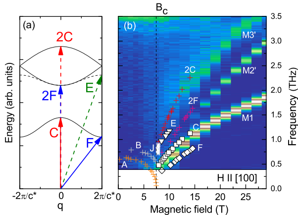
FIG. 5. (a) Proposed schematic energy diagram for \alpha -RuCl 3 in an arbitrary magnetic field above B_c . The modes C and F are single-magnon excitations, while the modes 2C and 2F correspond to two-magnon excitations. The mode E corresponds to an excitation of a two-magnon bound state. (b) Frequency-field dependences of selected ESR modes [from Figs. 2(a) 2(b)] and the color contour plot of the high-field Raman-scattering intensity [21] ( H \parallel [100] ).
