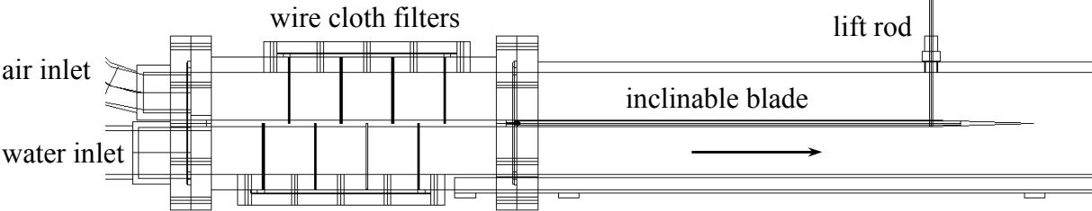
Fig. 2: The inlet device
