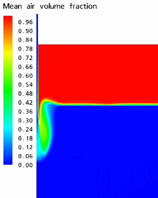
Fig. 4: Time averaged values of the gas volume fraction in case of the CFX-10 calculation
