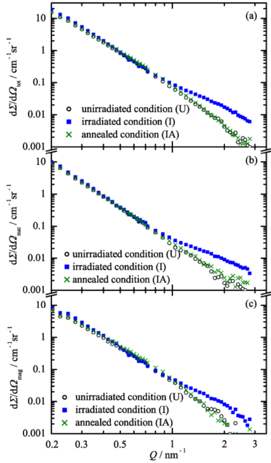
Fig. 1: Coherent neutron scattering cross section for unirradiated and irradiated conditions and after post-irradiation annealing; (a) total cross section, d\Sigma/d\Omega_{tot} , (b) nuclear cross section d\Sigma/d\Omega_{nuc} , (c) magnetic cross section d\Sigma/d\Omega_{mag} .
