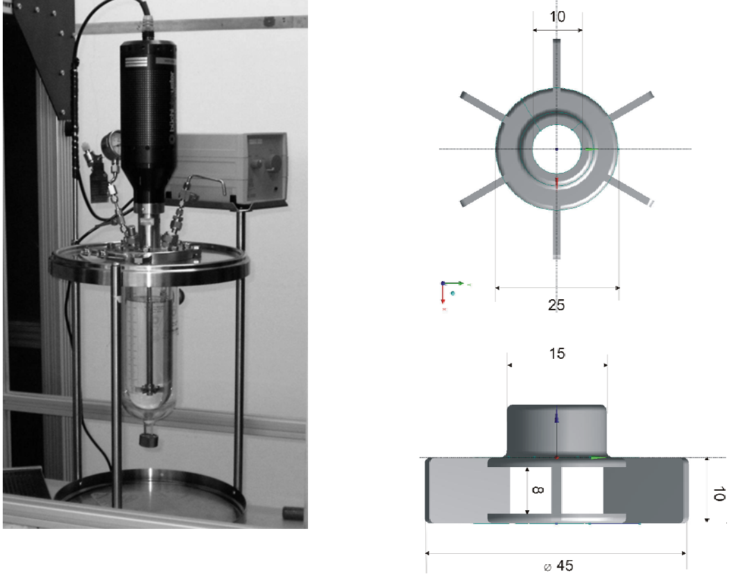
Fig. 2: Stirred tank reactor and stirrer geometry.
