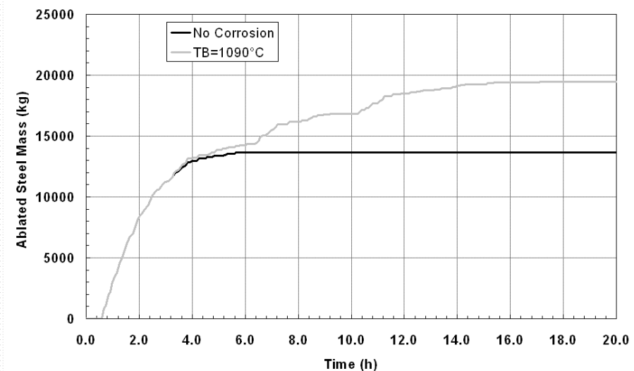
Fig. 5: Ablation kinetics (steel mass eroded from the RPV wall over time); grey with corrosion damage consideration, black without.
