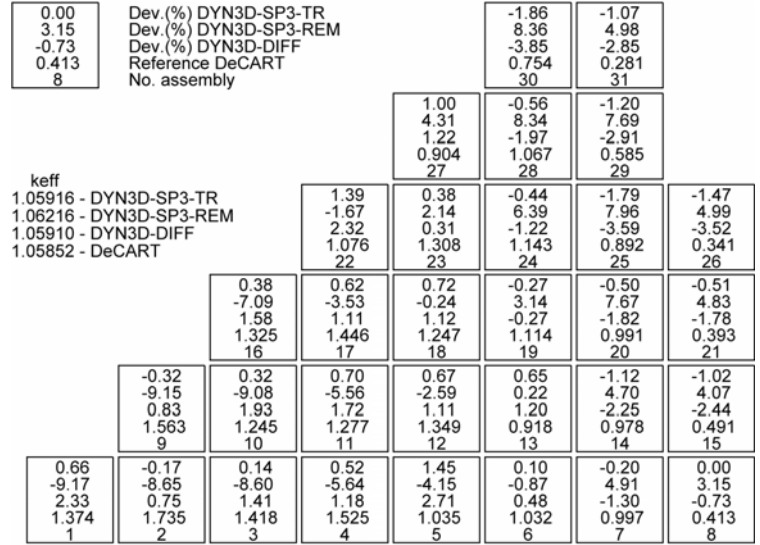
Fig. 3: Comparisons of the assembly powers of the three DYN3D calculations with the DeCART reference solution.
