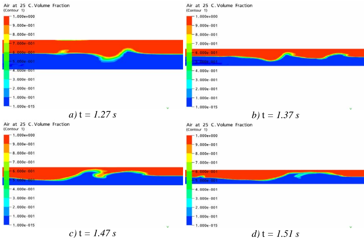
Fig. 7: Details of the slug generation calculated with ANSYS CFX at different simulation time
