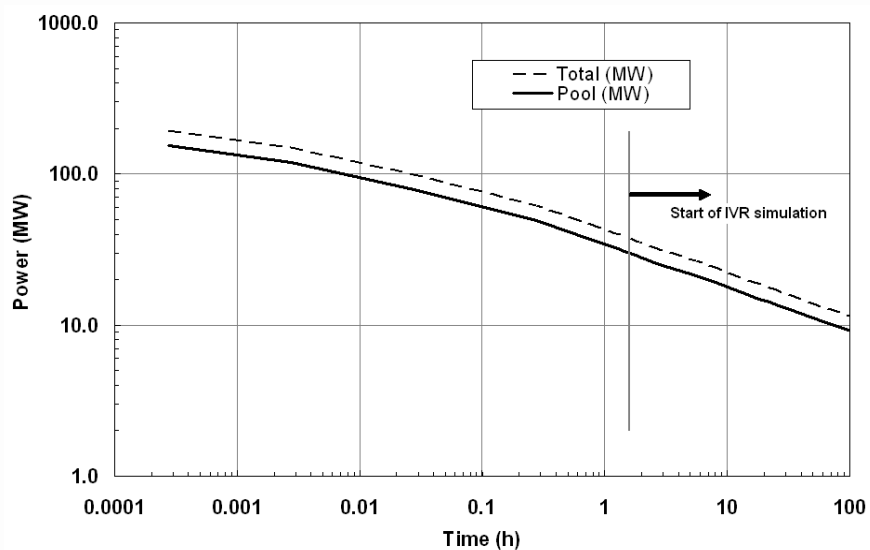
Fig. 4: Decay heat generation in the melt pool (VVER-1000).
