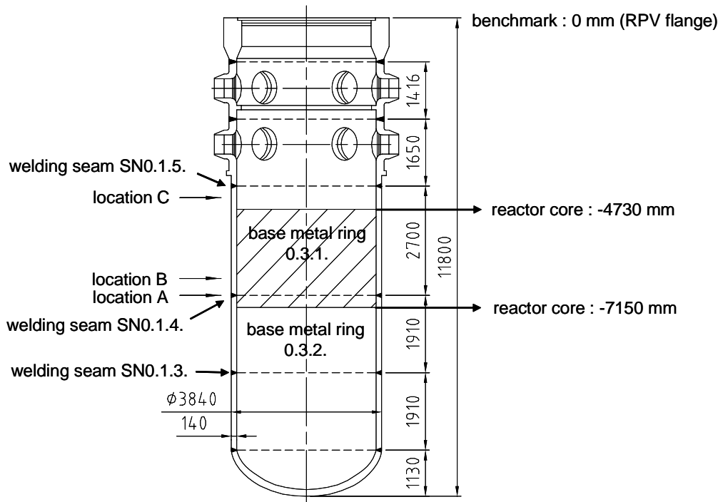
Fig. 3: RPV VVER 440 Greifswald Unit 1 and locations of the sampled trepans
