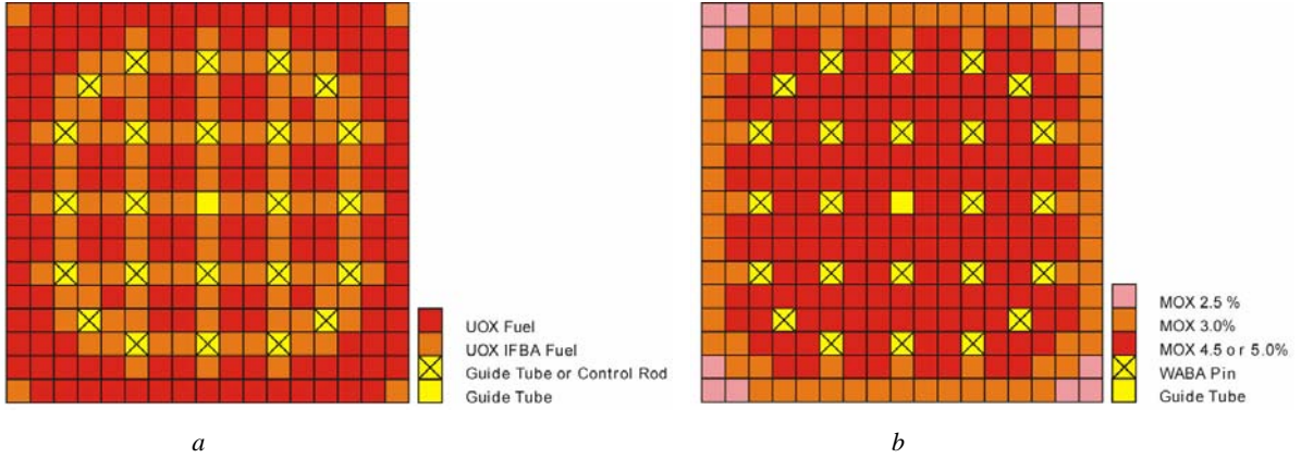
Fig. 2: Structure of the \text{UO}_2 assembly (a) and the MOX assembly (b).
