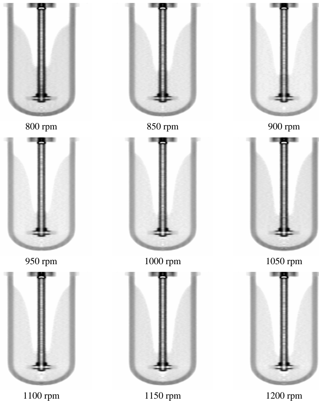
Fig. 3: Axial and radial fluid distribution in the stirred tank reactor measured with gamma ray CT.
