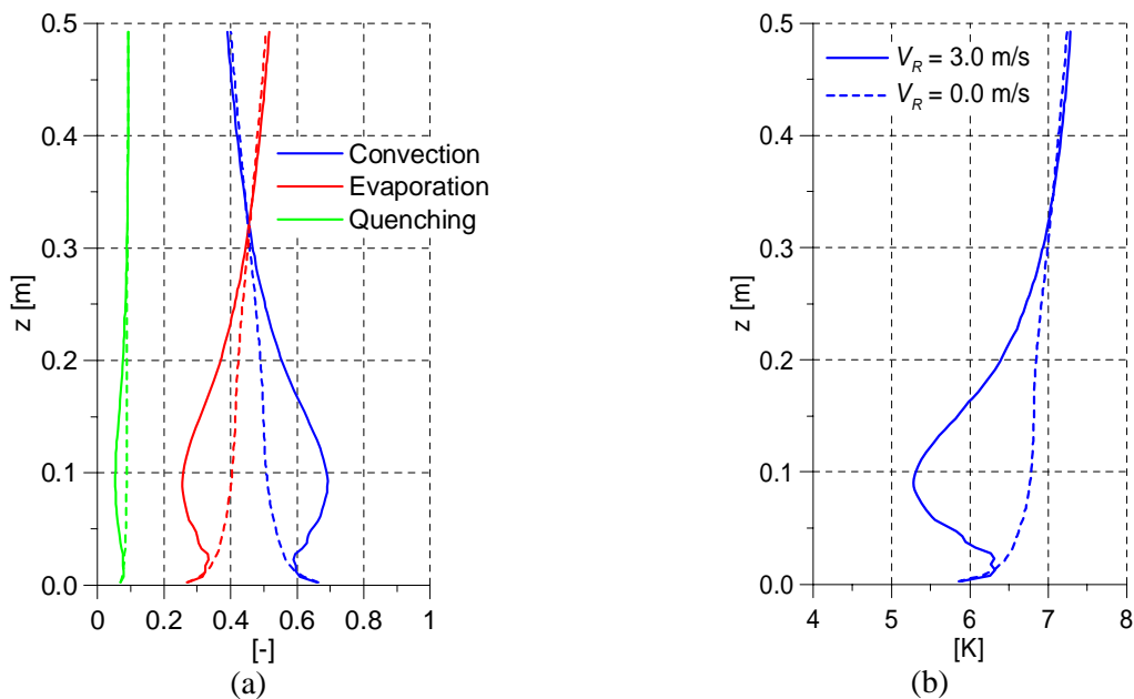
Fig. 7: Cross sectional averaged heat flux components (a) and superheating temperature at the rod surface (b) for the case d) (solid lines) and the reference case a) without swirl (dotted lines)
