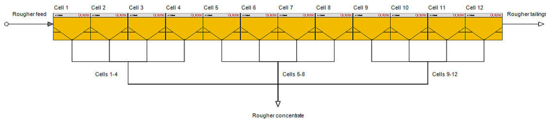
Figure 1: Streams involved in the rougher flotation bank analysis
