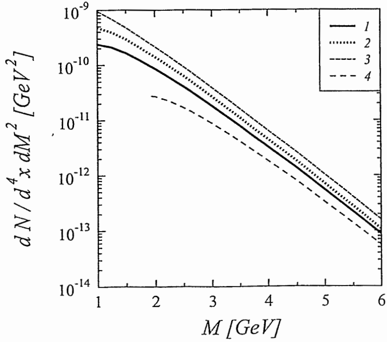
Fig. 2: The diphoton rates eq. (6) as function of the invariant mass for two temperatures (a: T = 250 MeV, b: T = 500 MeV) and \lambda_g = 0.5 and \lambda_q = \frac{1}{5}\lambda_g (the meaning of the curves is as in fig. 1).
