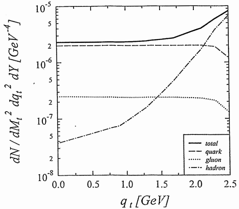
Fig. 6: Transverse momentum spectrum of diphotons for RIIC conditions for transverse pair mass M_{\perp} = 2.6 GeV (a: equation of state with reduced latent heat, b: standard bag model equation of state). Notation and initial conditions as for fig. 5.
