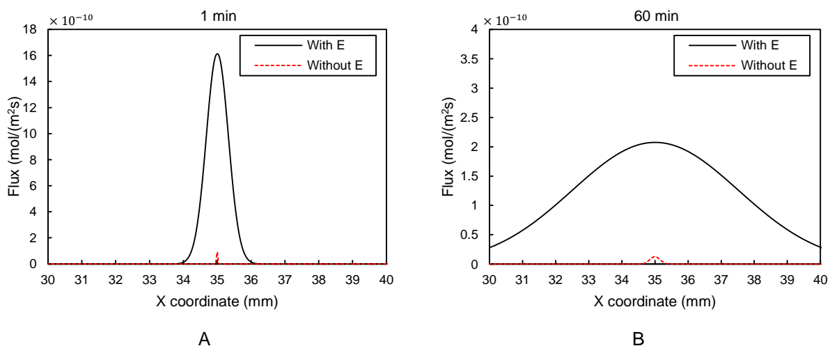
Figure 12. Flux of XG with and without electric field E at times of A) 1 min and B) 60 min.
