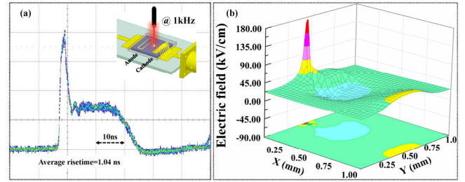
Fig.5. (a)1-kHz repetitive superposed waveforms at 80 kV/cm (Y/div 1V, X/div 10 ns), attenuated by 60 dB. The average risetime is about 1.04ns. The inset is the trigger sketch of PCSS (b) Transient electric field distribution at the time=1 ns for pulsed optical excitation with 9 ns FWHM centered at t=0 . X is the direction from anode to cathode and Y is direction parallel to the contacts.
