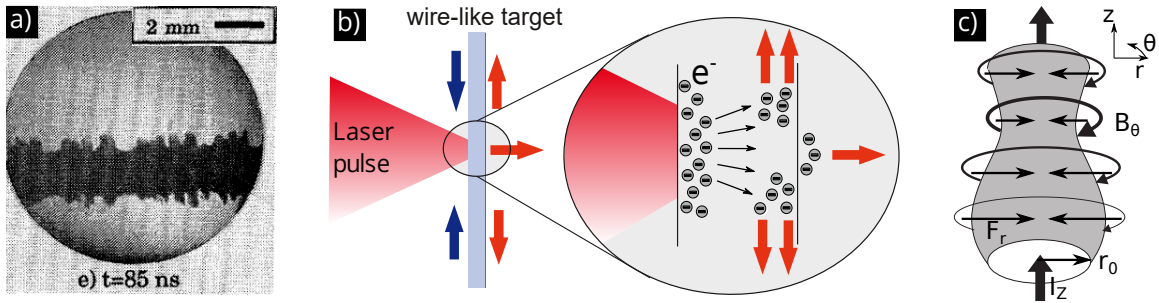
Figure 5.5: a) From Kalantar et al. [230]. A schlieren image of an aluminum wire (initial diameter of 100 \mu\text{m} ) recorded at the peak of a 350 kA current pulse of \sim 100 \text{ ns} duration shows modulations in the target diameter due to MHD instabilities. Note the much longer temporal and much larger spatial scale in comparison to the experimental results in figure 5.3. b) Model of the femtosecond dynamic of the irradiated wire-like target. Laser accelerated hot electrons (red arrow) leaving the interaction region are compensated by cold (blue arrow) return currents. c) Scheme of the m=0 MHD instabilities formation due to a pinching magnetic field generated by a current flow along the wire axis.
