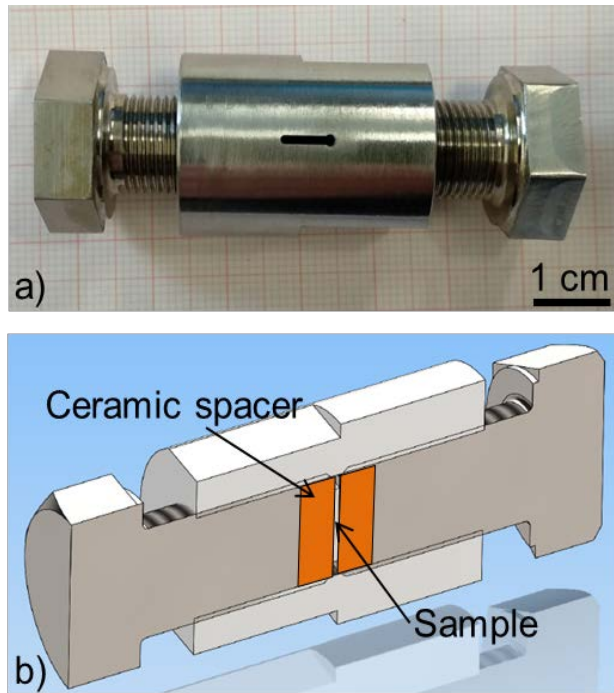
Fig. 1: (a) Pressure assembly, (b) cross-section schematic of the pressure assembly.
