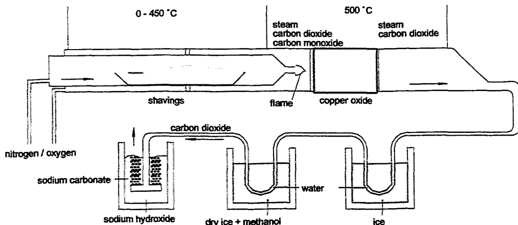
Fig. 1 Combustion furnace
