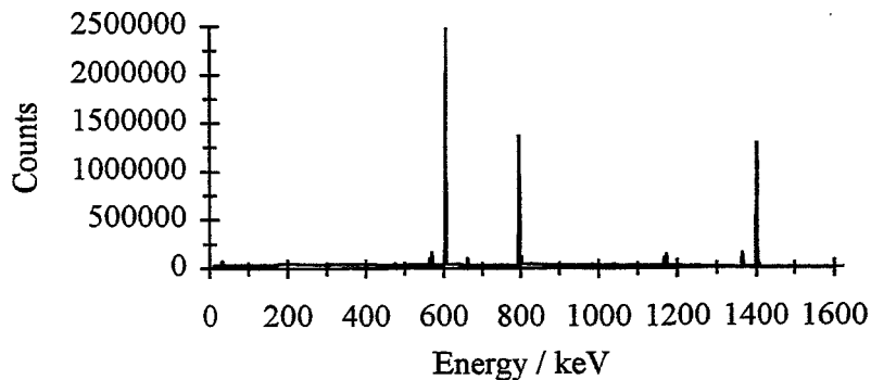
Figure 1: Spectrum of a ^{134}\text{Cs} standard solution in a plastic vial measured in a well-type detector for 1 day.
