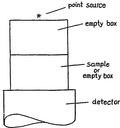
Fig. 2: Measuring geometry for absorption measurements
