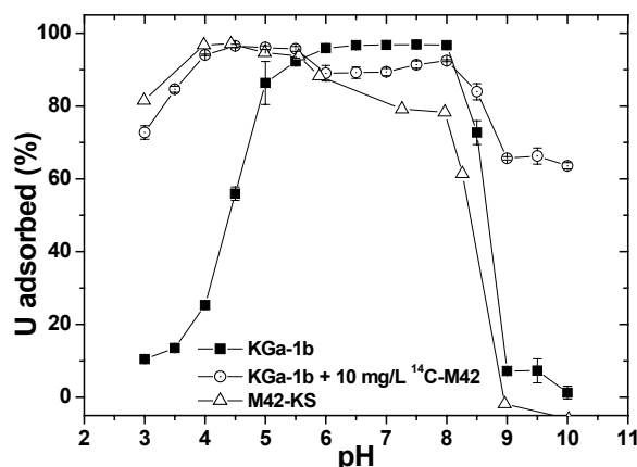
Fig. 2: U(VI) sorption onto the humic substance-kaolinite sorbate M42-KS and onto kaolinite (KGa-1b) in absence and presence of HA ^{14}C -M42 [2].
