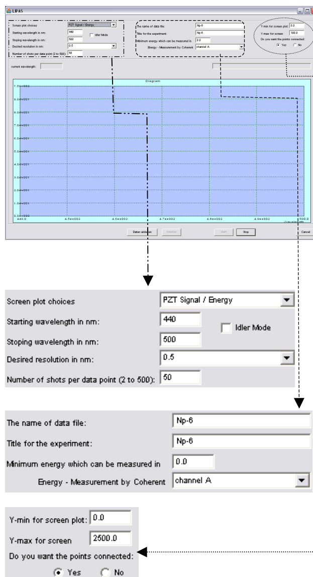
Fig. 2: Program software.
