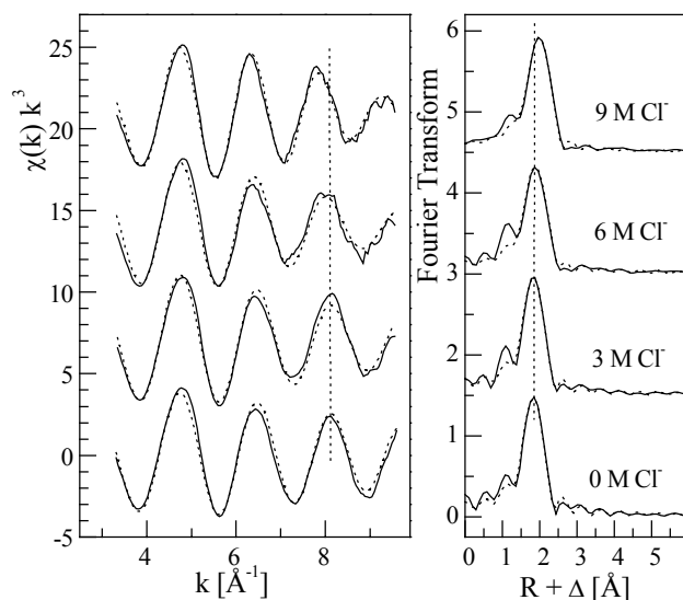
Fig. 1: U L_{III} -edge k^3 weighted EXAFS data (left) and corresponding Fourier transforms (right, 3.2 \leq k \leq 9.6 \text{ \AA}^{-1} ) of U(IV) at different Cl^- concentrations. Curve fits are shown as dotted lines.
