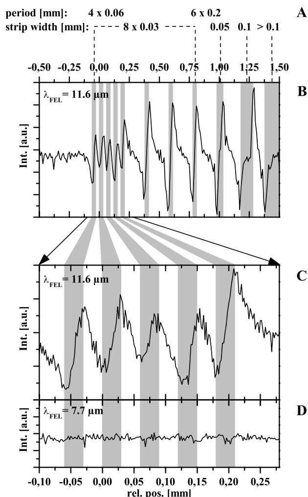
Fig. 2: Dimensions of the implantation pattern for the preparation of the Ge-substrate with \text{O}^+ -ions (A). Extracted absorption profiles from the maximum of the deflection curves (B–D): Profile (step width: 10 \mu\text{m} ) of the whole implanted structure (B). Profiles (step width: 2 \mu\text{m} ) of five thin lines at different FEL wavelengths (C–D) with max. absorption (C) and no absorption (D).
