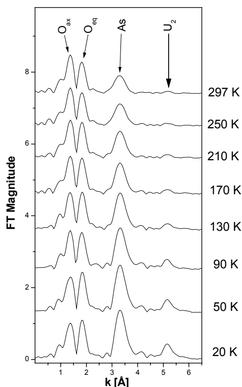
Fig. 1: Fourier transform of the U L_{\text{III}} -edge k^3 -weighted EXAFS data ( 3.2 \leq k \leq 15.7 \text{ \AA}^{-1} ).
