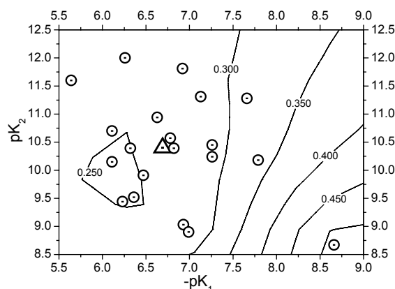
Fig. 2: Randomly distributed pK of hematite ( \circ : varied pK , \Delta : exp. mean pK ) plotted in a surface of the resulting \Sigma \text{abs}(\Delta \log K_D)/n (see numbers on the contour-lines).
