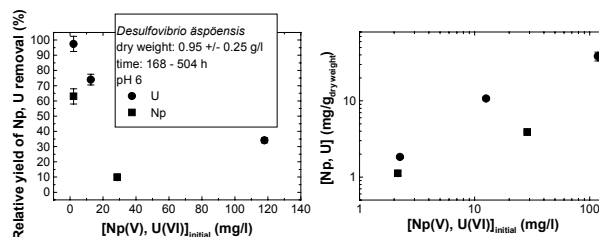
Fig. 3: Removed neptunium/uranium from the solution in the presence of D. äspöensis at pH 6.
