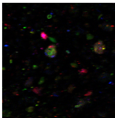
Fig. 2: F3 \mu -XRF map ( 400 \times 400 \mu\text{m}^2 ). U (red), Cu (green), V (blue).
