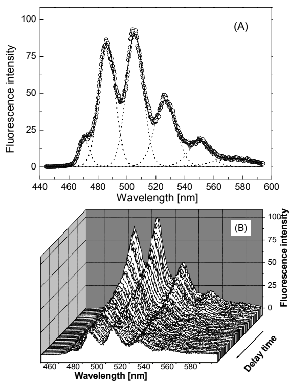
Fig 1: Fluorescence emission bands of andersonite (A). (The dotted lines show the curve fit of the spectra Gaussian shapes.) Fluorescence spectra of synthetic andersonite as a function of delay time (B).
