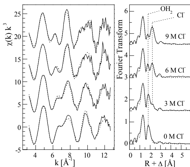
Fig. 1: U L III -edge k^3 weighted EXAFS data (left) and corresponding Fourier transforms (right, 3.2 \leq k \leq 12.7 \text{ \AA}^{-1} ) of UO 2 2+ at four different Cl - concentrations. Curve fits are shown as dotted lines.
