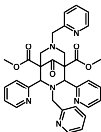
Fig. 1: Structure of hexadentate bispidine (N2Py4).
