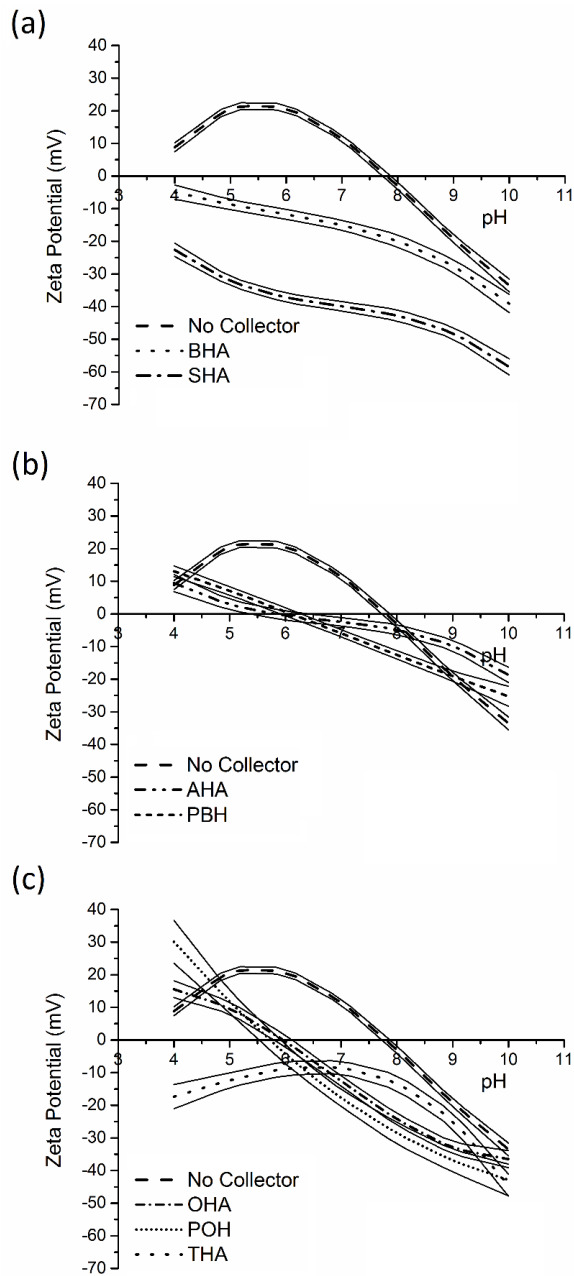
Figure 4 Zeta potential trend of malachite in the presence and absence of (a) aromatic, (b) short chain alkyl ( C_2 and C_4 ) and (c) long chain alkyl ( C_8 and C_{14} ) hydroxamates at a concentration of 1.7 \times 10^{-3} mol/ton (Error intervals shown are 95 % confidence intervals)
